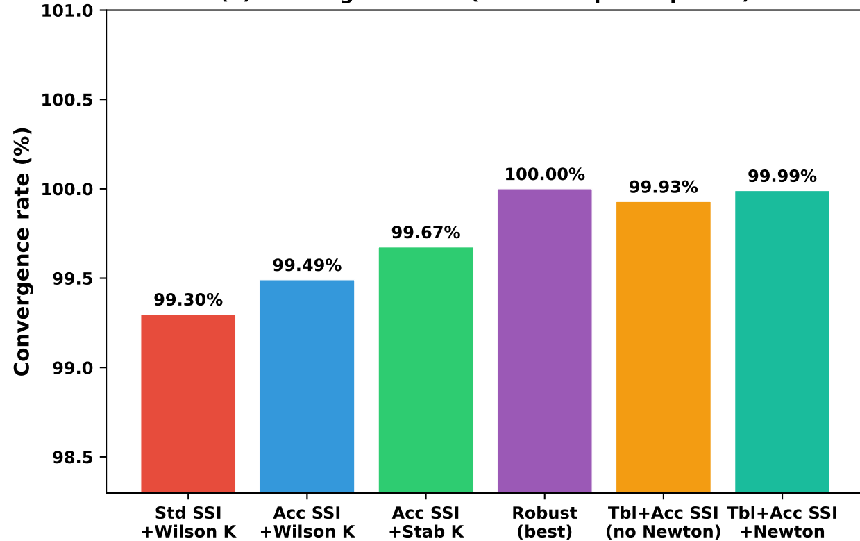
(a) Convergence rate (9825 two-phase points)
