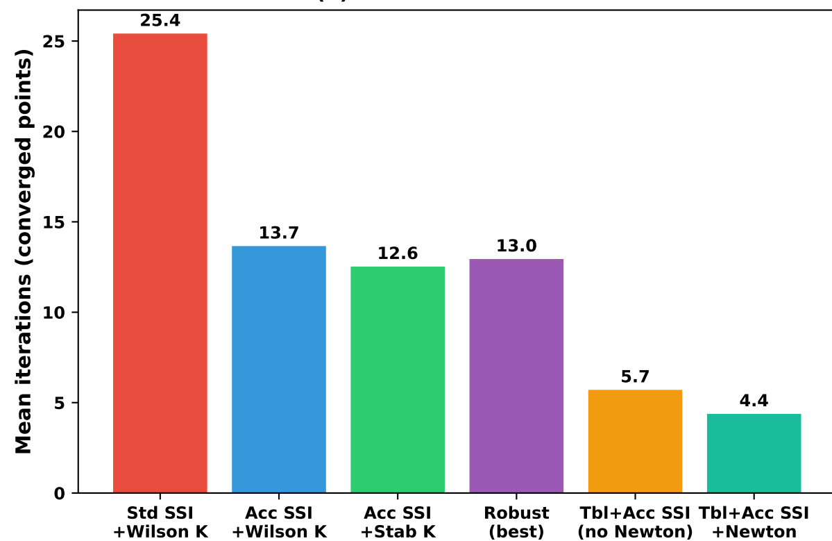
(b) Mean total iterations
