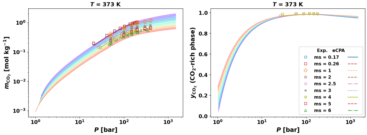
Figure S3: CO 2 + NaCl brine phase equilibria at T = 100\text{ }^{\circ}\text{C} for which both CO 2 molality m_{\text{CO}_2} (left panel) and CO 2 mole fraction in the CO 2 -rich phase y_{\text{CO}_2} (right panel) data are available. Open symbols: experimental data (Bando et al., 2003; Chabab et al., 2020; Guo et al., 2015; Hou et al., 2013; Koschel et al., 2006; Liu et al., 2021; Messabeb et al., 2016; Savary et al., 2012; Takenouchi and Kennedy, 1965; Yan et al., 2011; Zhao et al., 2015); discrete lines with markers: eCPA at the experimental NaCl molalities. Rainbow-colored background bands: continuous eCPA predictions across m_s = 0 – 6 mol kg -1 (color scale as in Fig. 1).
