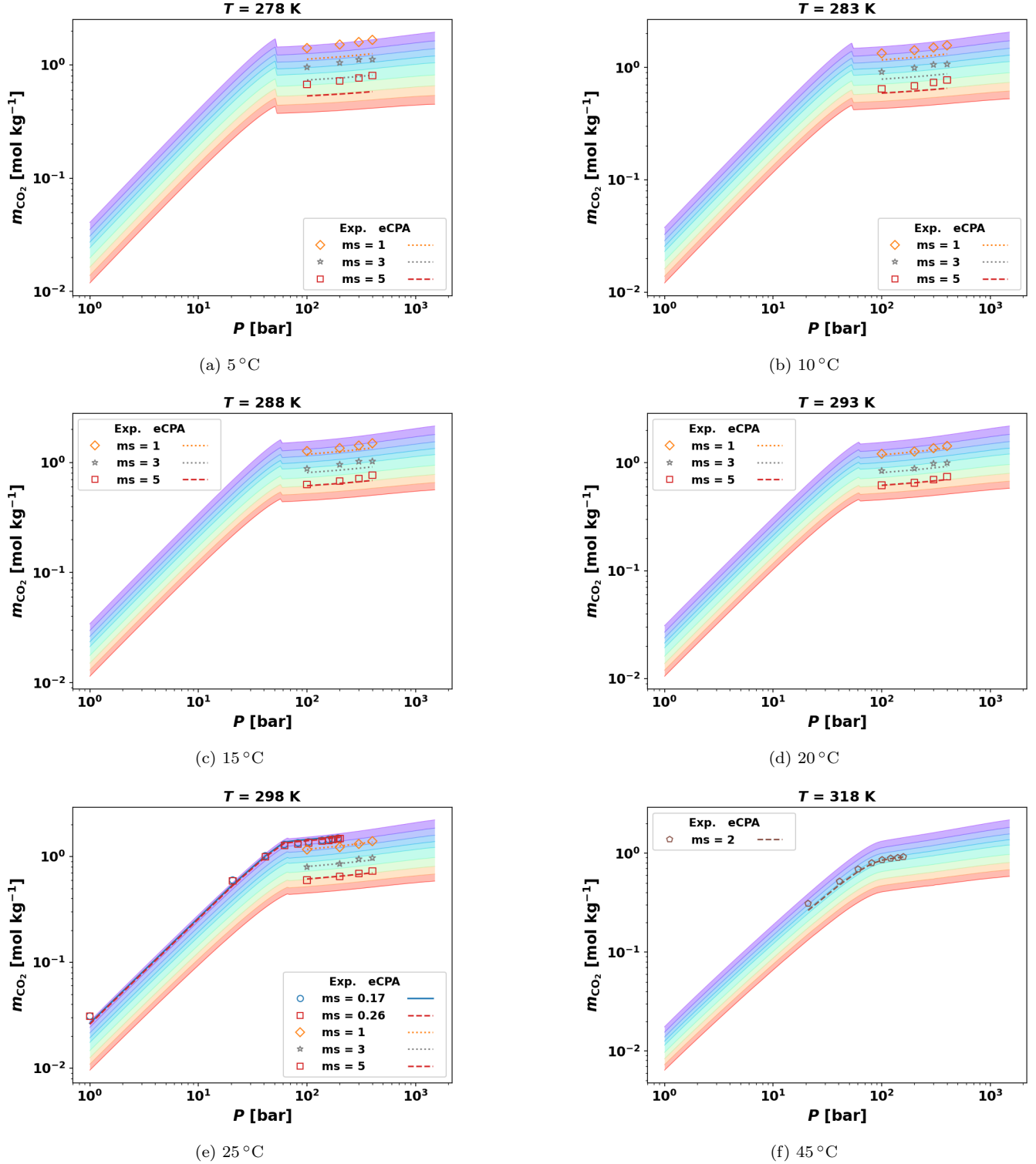
Figure S2: CO 2 solubility in NaCl brine at thirteen temperatures not shown in Fig. 2 (5–350 °C), including data at high NaCl molalities up to m_s = 6 mol kg -1 from multiple sources. Each panel shows CO 2 molality m_{\text{CO}_2} [mol kg -1 ] vs. pressure (log-log). Open symbols: experimental data (Guo et al., 2015; Rumpf et al., 1994; Bando et al., 2003; Chabab et al., 2020; Liu et al., 2021, 2011; Nighswander et al., 1989; Takenouchi and Kennedy, 1965; Yan et al., 2011); discrete lines with markers: eCPA at the experimental NaCl molalities. Rainbow-colored background bands: continuous eCPA predictions across m_s = 0 –6 mol kg -1 (color scale as in Fig. 1). At T \geq 400 °C, eCPA predicts single-phase (fully miscible) behavior for all available experimental pressures.
