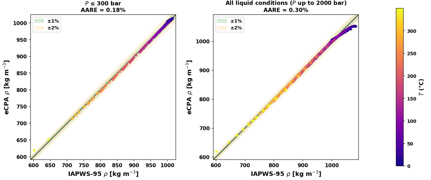
Figure S5: Parity plot: eCPA pure-water density versus IAPWS-95 (Wagner and Pruß, 2002) (475 liquid/compressed-water conditions, T = 0\text{--}350\text{ }^{\circ}\text{C} , P = 1\text{--}2000\text{ bar} ). Left panel: P \leq 300\text{ bar} ; right panel: all conditions up to 2000 bar. Points are colored by temperature; shaded bands indicate \pm 1\% and \pm 2\% deviations. The temperature-dependent Péneloux shift (Section S2) is applied.
