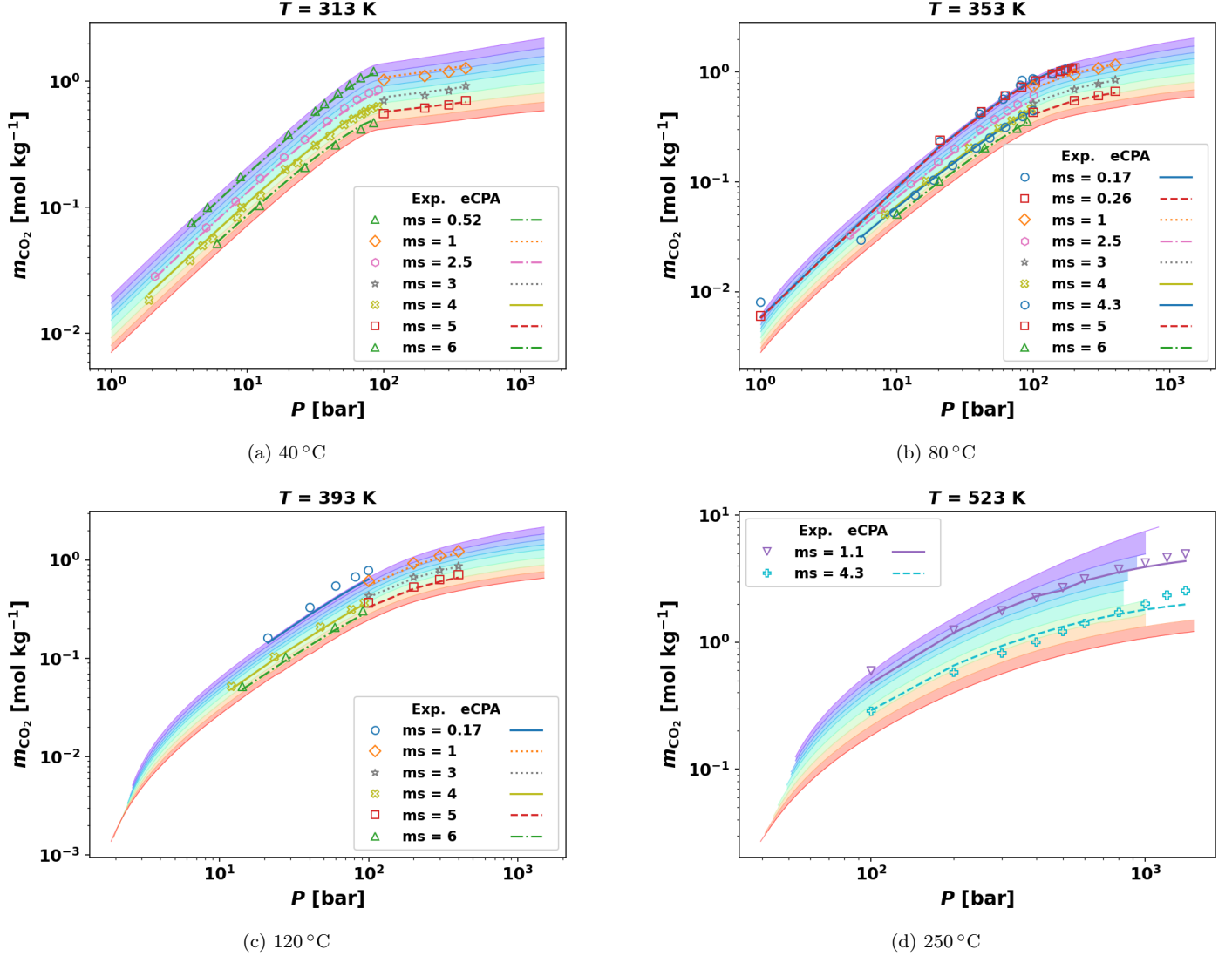
Figure 2: CO 2 solubility in NaCl brine at four representative temperatures (40, 80, 120, and 250 °C). Each panel shows CO 2 molality m_{\text{CO}_2} [mol kg -1 ] vs. pressure (log-log). Open symbols: experimental data (Guo et al., 2015; Rumpf et al., 1994; Kiepe et al., 2002; Nighswander et al., 1989; Bando et al., 2003; Liu et al., 2021; Takenouchi and Kennedy, 1965); discrete lines with markers: eCPA at the experimental NaCl molalities. Rainbow-colored background bands: continuous eCPA predictions spanning m_s = 0 –6 mol kg -1 (color scale as in Fig. 1: violet \approx 0 , red = 6 mol kg -1 ). Temperatures with additional CO 2 -rich phase data ( y_{\text{CO}_2} ) are shown separately in Fig. 3; all 18 temperatures in Figs. S2 and S3.
