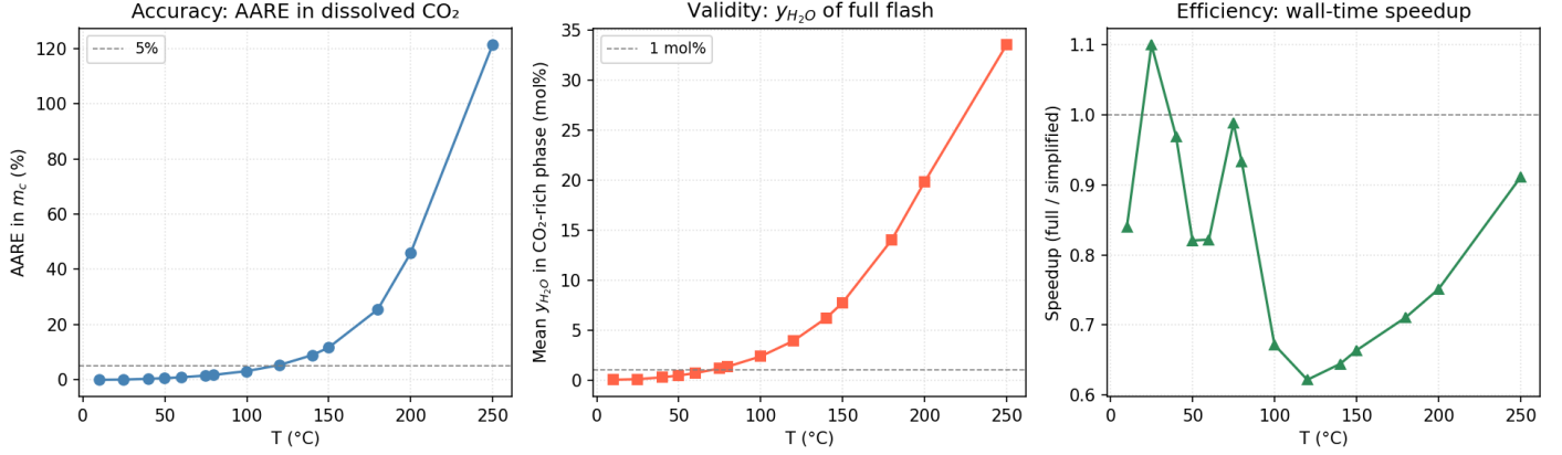
Figure S8: Simplified flash benchmark over 3,285 two-phase conditions ( P = 25\text{--}800 bar; z_{\text{CO}_2} = 0.01\text{--}0.70 ; m_s = 1\text{--}6 mol kg -1 ). Left: AARE in dissolved CO 2 molality m_{\text{CO}_2} as a function of temperature; the dashed line marks 5%. Middle: mean H 2 O mole fraction in the CO 2 -rich phase from the full flash, which directly quantifies the magnitude of the y_{\text{H}_2\text{O}} = 0 assumption; dashed line at 1 mol%. Right: ratio of mean full-flash wall time to simplified-flash wall time; the two methods are essentially iso-cost across all temperatures.
