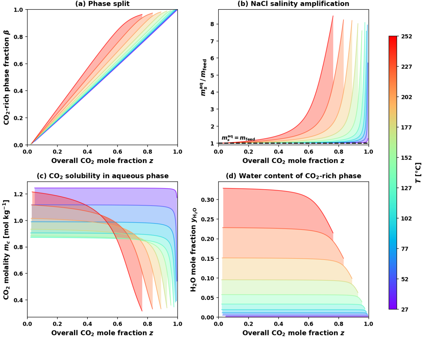
Figure 4: eCPA flash results as a function of overall CO 2 feed mole fraction z_{\text{CO}_2} at P = 200 bar, feed molality m_s = 1.0 \text{ mol kg}^{-1} NaCl, and ten isotherms from 27 to 252 °C (violet to red). (a) CO 2 -rich phase fraction \beta ; the two-phase window narrows progressively at higher temperature. (b) Ratio of equilibrium aqueous NaCl molality to feed molality, m_s^{\text{aq}}/m_s ; NaCl concentrates in the aqueous phase as H 2 O partitions to the CO 2 -rich phase, reaching a factor of \sim 8 at T = 252 °C and z_{\text{CO}_2} \approx 0.98 . (c) CO 2 molality m_{\text{CO}_2} in the aqueous phase; the salting-out effect driven by the elevated m_s^{\text{aq}} reduces CO 2 solubility with increasing z_{\text{CO}_2} . (d) H 2 O mole fraction y_{\text{H}_2\text{O}} in the CO 2 -rich phase; substantial water content at high temperatures (up to \sim 30 mol% at 252 °C) and its strong variation with z_{\text{CO}_2} highlight the need for full flash rather than a fixed-salinity VLE lookup.
