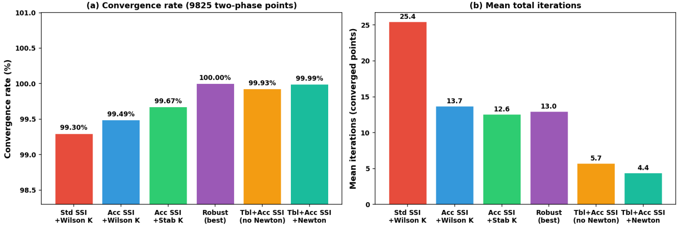
Figure S11: CPA flash strategy comparison across all 9,825 two-phase conditions of the salt-free CO 2 + H 2 O parameter-space scan ( T = 0-425^\circ\text{C} , P = 1-1500 bar, z_{\text{CO}_2} = 0.001-0.999 ). (a) Convergence rate; (b) mean total iterations (converged points only). Strategies are ordered from simplest cold-start (standard SSI with Wilson K) to the most optimized (table warm-start with SSI and Newton polish). The final strategy achieves a 73% reduction in mean iterations relative to the standard cold-start baseline.
