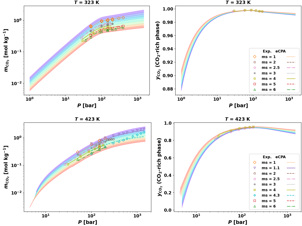
Figure 3: \text{CO}_2 + \text{NaCl} brine phase equilibria at temperatures for which both \text{CO}_2 molality ( m_{\text{CO}_2} , left panel) and \text{CO}_2 mole fraction in the \text{CO}_2 -rich phase ( y_{\text{CO}_2} , right panel) data are available: (top) 50\text{ }^\circ\text{C} , (bottom) 150\text{ }^\circ\text{C} (see also Fig. S3 for 100\text{ }^\circ\text{C} ). Open symbols: experimental data (Bando et al., 2003; Chabab et al., 2020; Guo et al., 2015; Hou et al., 2013; Koschel et al., 2006; Liu et al., 2021; Messabeh et al., 2016; Savary et al., 2012; Takenouchi and Kennedy, 1965; Yan et al., 2011; Zhao et al., 2015); discrete lines with markers: eCPA at the experimental NaCl molalities. Rainbow-colored background bands: continuous eCPA predictions across m_s = 0\text{--}6\text{ mol kg}^{-1} (color scale as in Fig. 1).
