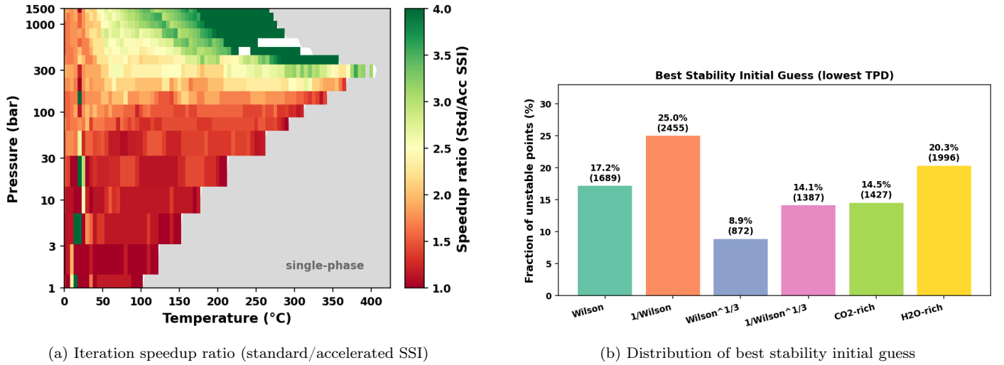
Figure 6: (a) Iteration speedup from accelerated SSI, averaged over z_{\text{CO}_2} (two-phase only). The speedup exceeds 2\times across most of the parameter space and reaches 3\text{--}4\times near the critical region. (b) Distribution of the initial guess that found the lowest TPD across all 9,825 unstable points. No single guess dominates: each of the six trials is the best for 9–25% of conditions, demonstrating the importance of multiple initial guesses for robust stability testing.
