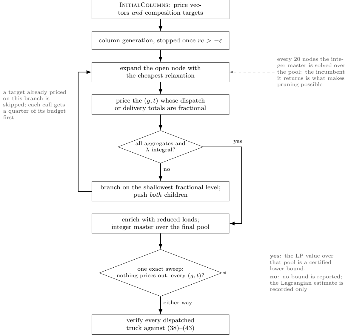
Figure 3: MATH-3D-SCPTOP end to end. Columns keep being generated after the branching decisions, which a price-and-branch scheme over a frozen pool cannot do. Two conventions are worth reading off the diagram: the incumbent comes from an integer master solved periodically over the pool rather than from the tree reaching integrality, and the bound is decided at a single point — either an exact sweep proves that nothing prices out anywhere, or no bound is reported at all.
