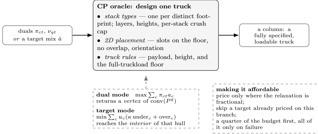
Figure 3: The pricing subproblem. Geometry, height, crush limits, payload and the full-truckload rule are enforced inside the oracle, so any column it returns is a physically loadable truck. In dual mode it maximises the dual-weighted load and therefore returns a vertex of \text{conv}(P^g) ; in target mode it minimises a volume-weighted asymmetric deviation from a wanted composition, which is how loads in the interior of that hull are obtained (Figure 4). Pricing accounted for 1451 of 1453 seconds of one search, so the measures on the right are what make a node affordable.
