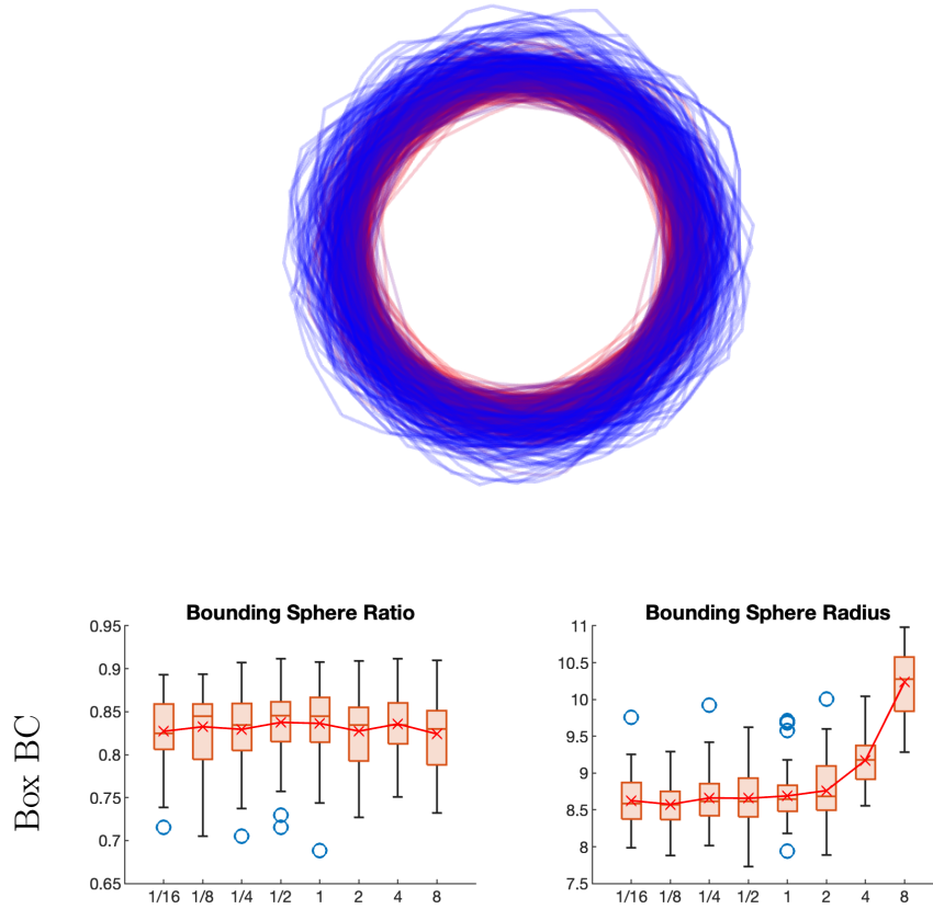
Figure 4: Convergence of Elliptic PDE solutions. Nutirent dependendent CCM. Convergence as space step is decreased. Dashes line is results from solving the PDE on a growing domain.
