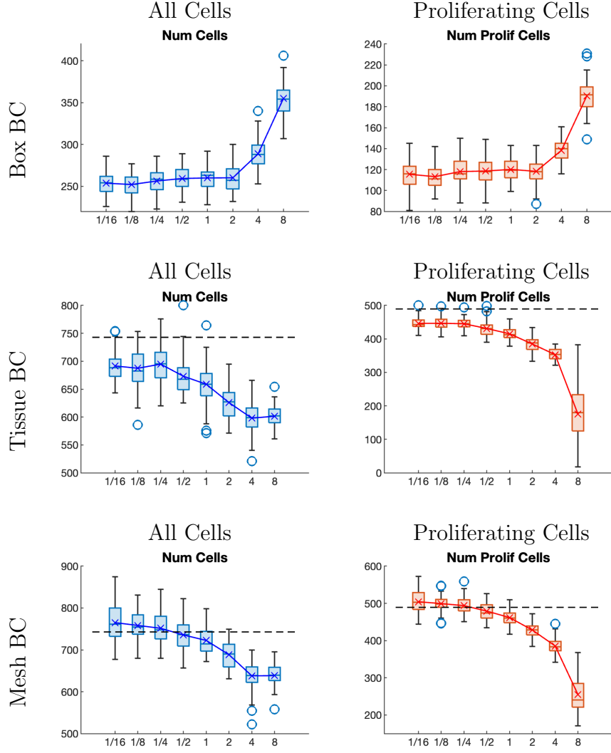
Figure 3: Convergence of Elliptic PDE solutions. Nutrient dependent CCM. Convergence as space step is decreased. Dashes line is results from solving the PDE on a growing domain.
