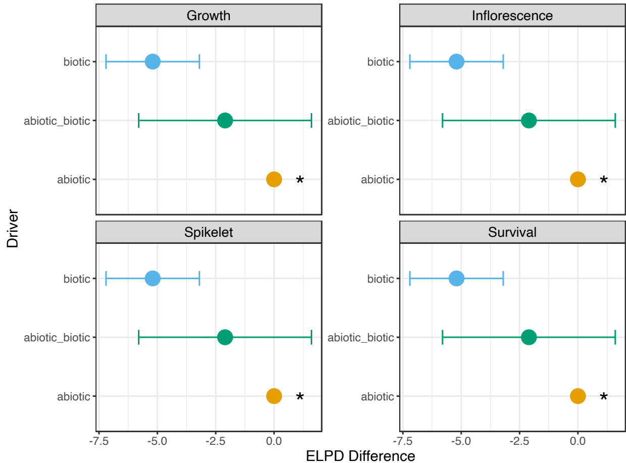
Figure 6: Model comparison across vital rates (survival, growth, flowering, spikelet production) using expected log predictive density (ELPD) differences. ELPD measures a model's ability to predict new data, with higher values indicating better predictive performance. Differences in ELPD relative to the best-supported model (abiotic-only) show which models perform better or worse. Circles indicate the ELPD of each model, error bars represent the standard error of the differences (SE), and stars mark the model with the highest ELPD.
