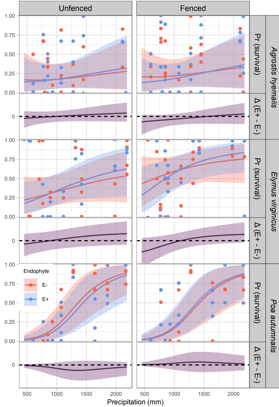
Figure 2: Predicted survival rate (top panels) and endophyte effect ( \Delta = E^+ - E^- , bottom panels) across precipitation gradients. Lines show posterior means for E^+ (blue) and E^- (red), with shading indicating 90% credible intervals. Points represent mean observed survival per plot, jittered for visualization. The dashed line at \Delta = 0 indicates no endophyte effect. Panels are organized by species (AGHY, ELVI, POAU) and herbivory treatment (Fenced, Unfenced).
