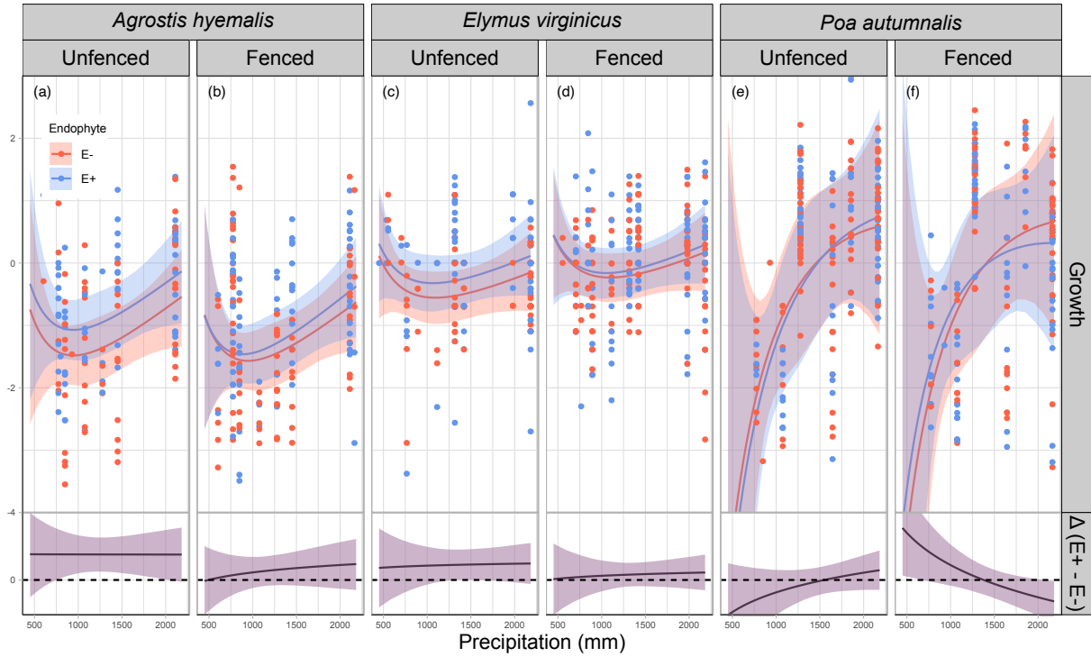
Figure 3: Predicted relative growth from year to the next year (top panels) and endophyte effect ( \Delta = E^+ - E^- , bottom panels) across precipitation gradients. Lines show posterior means for E^+ (blue) and E^- (red), with shading indicating 90% credible intervals. Points represent mean observed growth per plot, jittered for visualization. The dashed line at \Delta = 0 indicates no endophyte effect. Panels are organized by species and herbivory treatment (Fenced, Unfenced).
