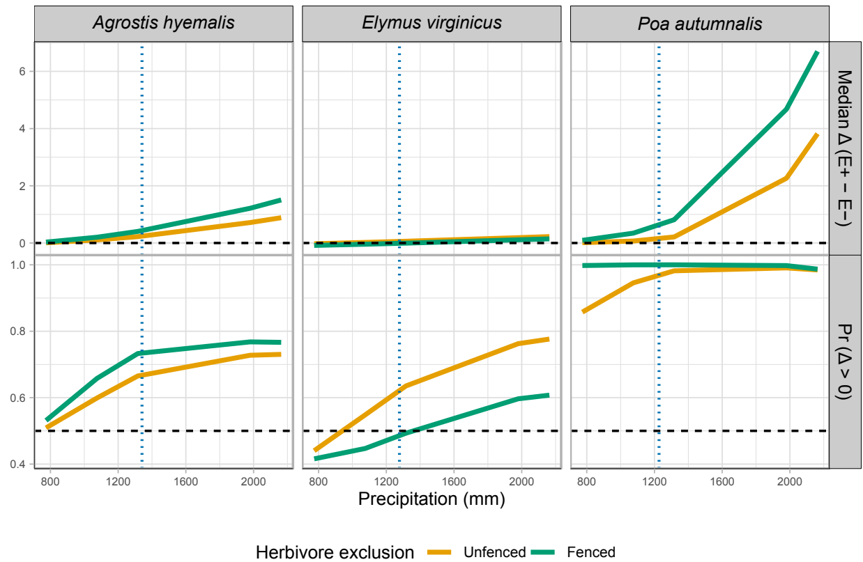
Figure S-5: Effects of endophyte infection on flowering output across a precipitation gradient for three cool-season grass species. Lines show the median posterior difference \Delta (E^+ - E^-) and the posterior probability that \Delta > 0 under fenced (herbivores excluded) and unfenced (herbivores present) conditions. Horizontal dashed lines indicate \Delta = 0 for median differences and \Pr(\Delta > 0) = 0.5 . Endophyte effects were generally positive for Agrostis hyemalis and Poa autumnalis , but for Elymus virginicus benefits were context-dependent, with costs at lower precipitation
