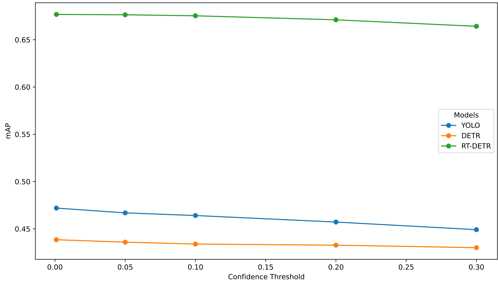
mAP (AP@[.5:.95])
