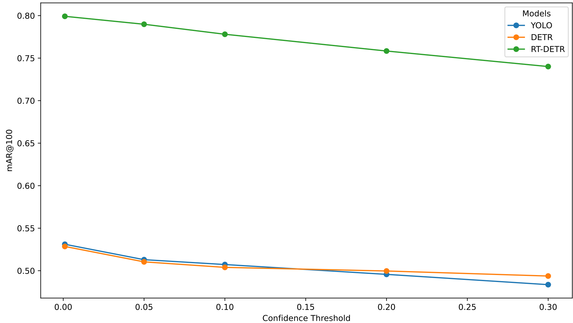
Recall: mAR@100
