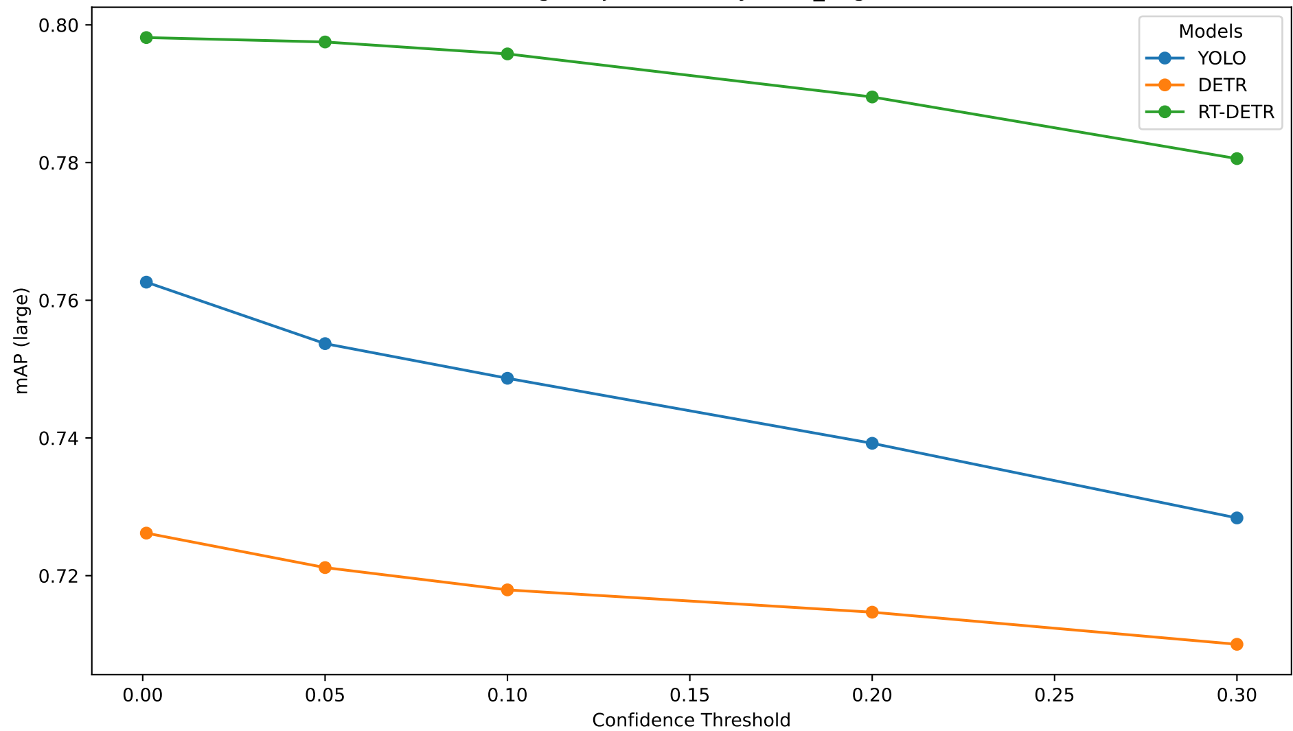
Large Object Accuracy: mAP_large
