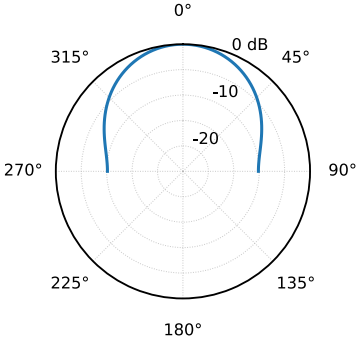
Directional response at 2000 Hz
