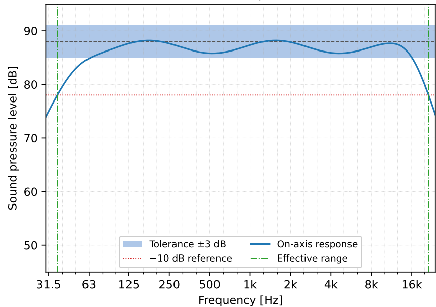
On-axis response
