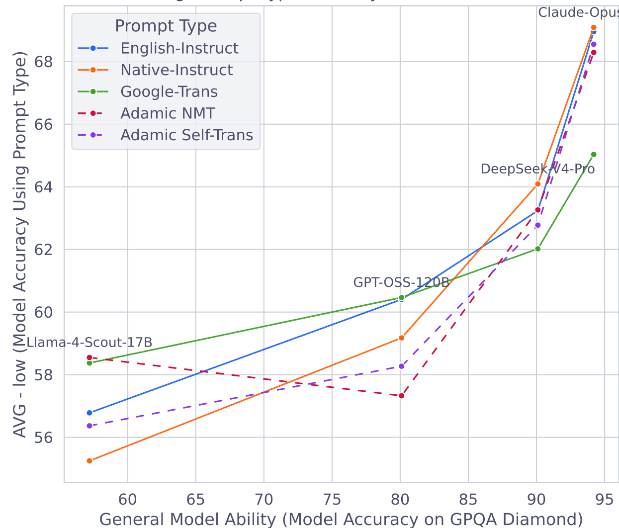
Low Resource Lang: Prompt Type Accuracy Relative to General Model Ability
