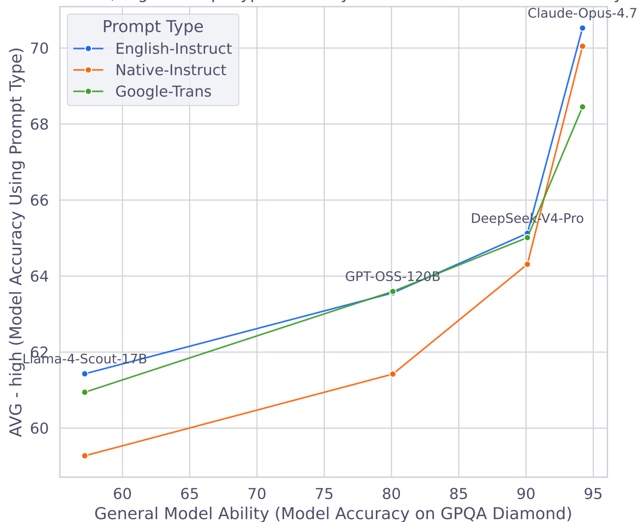
Focused, High: Prompt Type Accuracy Relative to General Model Ability
