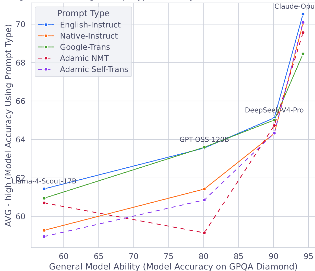
High Resource Lang: Prompt Type Accuracy Relative to General Model Ability
