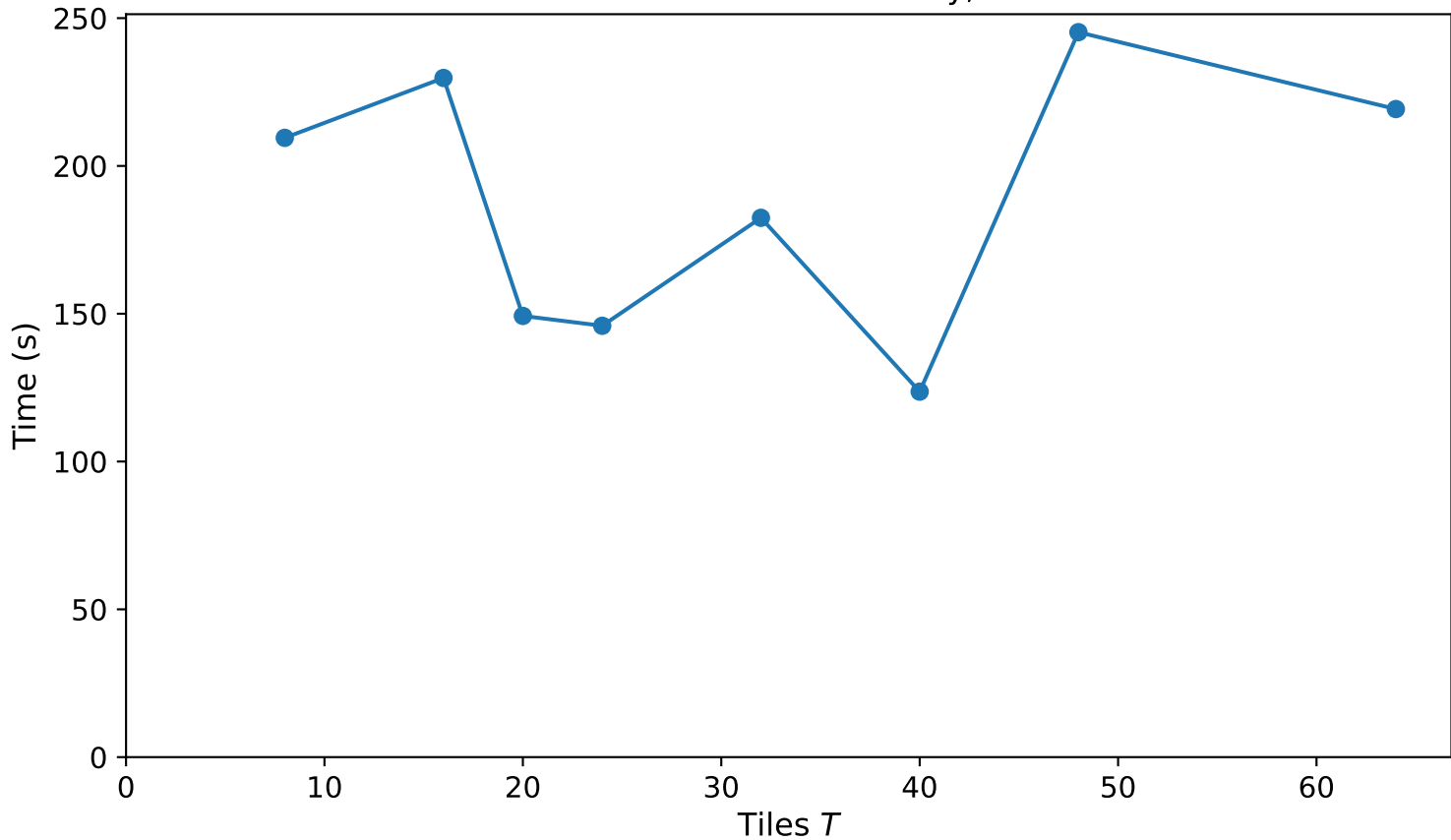
Tiles vs. executiontime: Cholesky, N=24000
