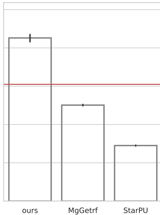
2GPUs
