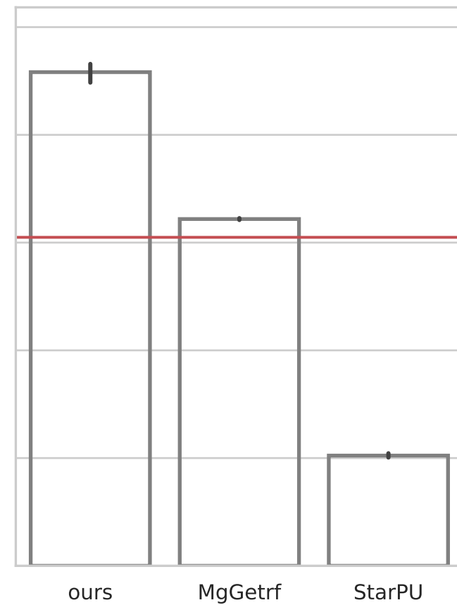
4GPUs
