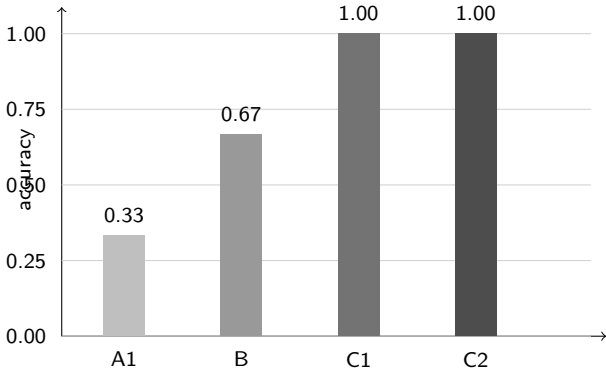
Structural-OOD accuracy
