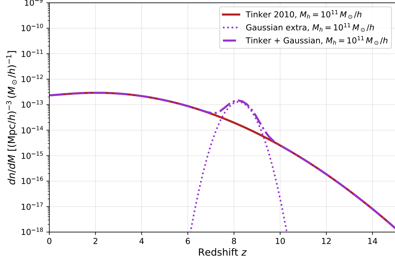
HMF vs z at M_h = 10^{11} M_{\odot}/h : z_0 = 8.2 , \sigma_z = 0.43
