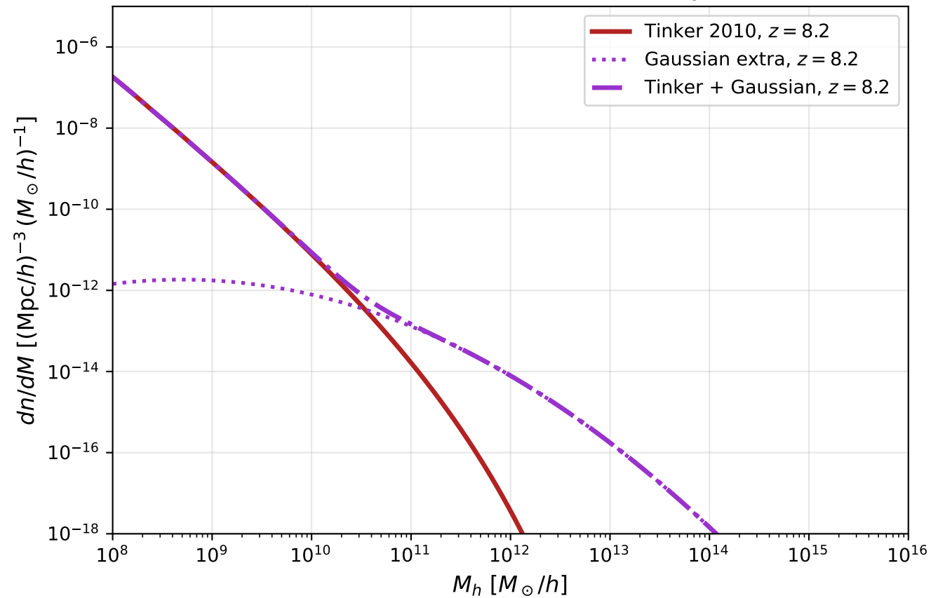
HMF at z = 8.2 : A = 0.013 , \log M_0 = 11.0 , \sigma_{\log M} = 1.0
