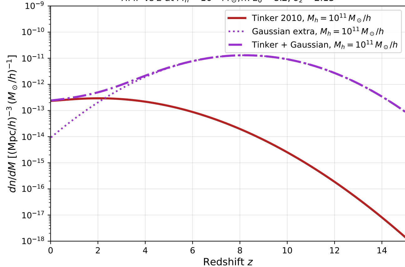
HMF vs z at M_h = 10^{11} M_\odot/h : z_0 = 8.2 , \sigma_z = 2.15
