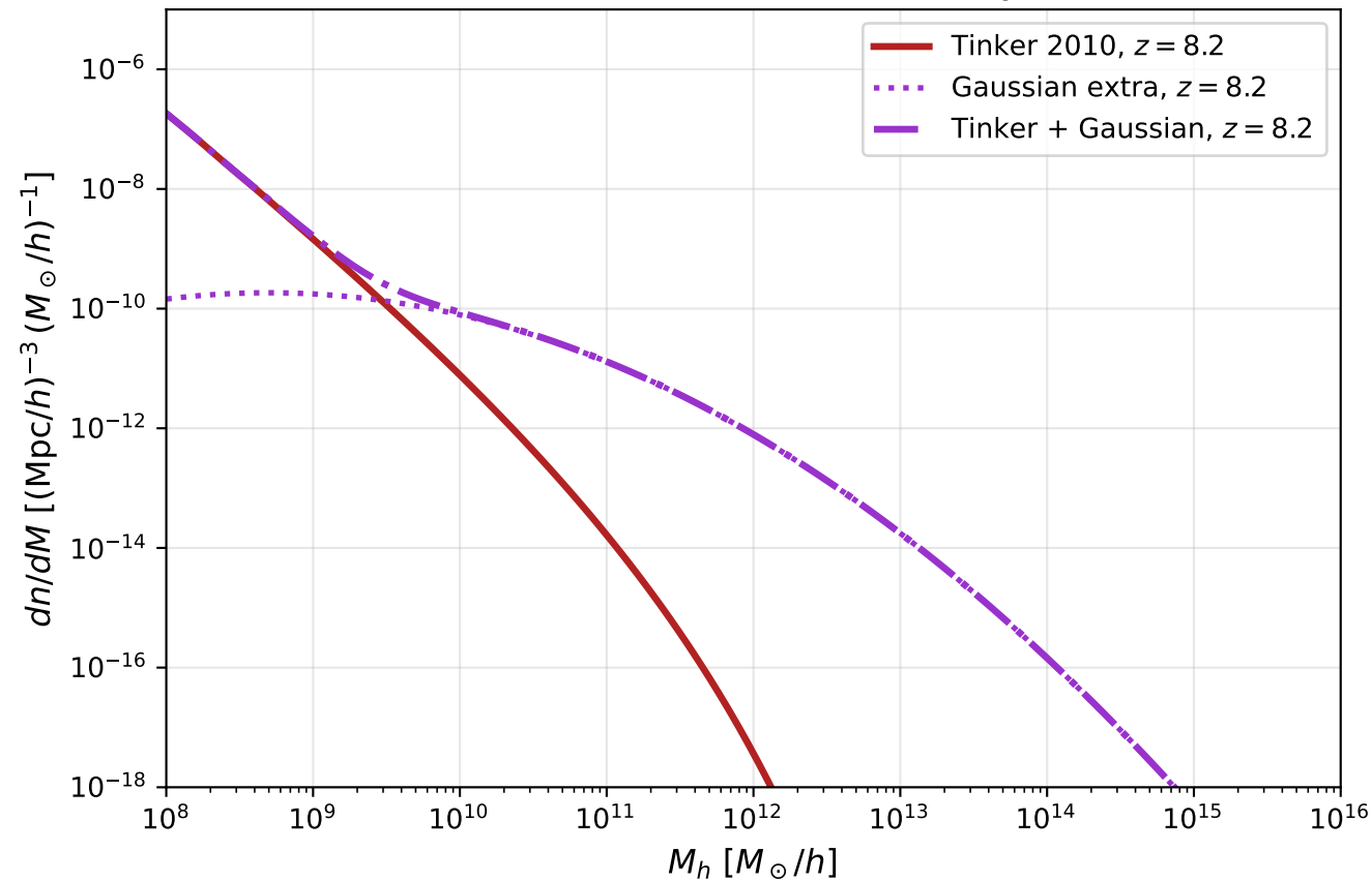
HMF at z = 8.2 : A = 1.3 , \log M_0 = 11.0 , \sigma_{\log M} = 1.0
