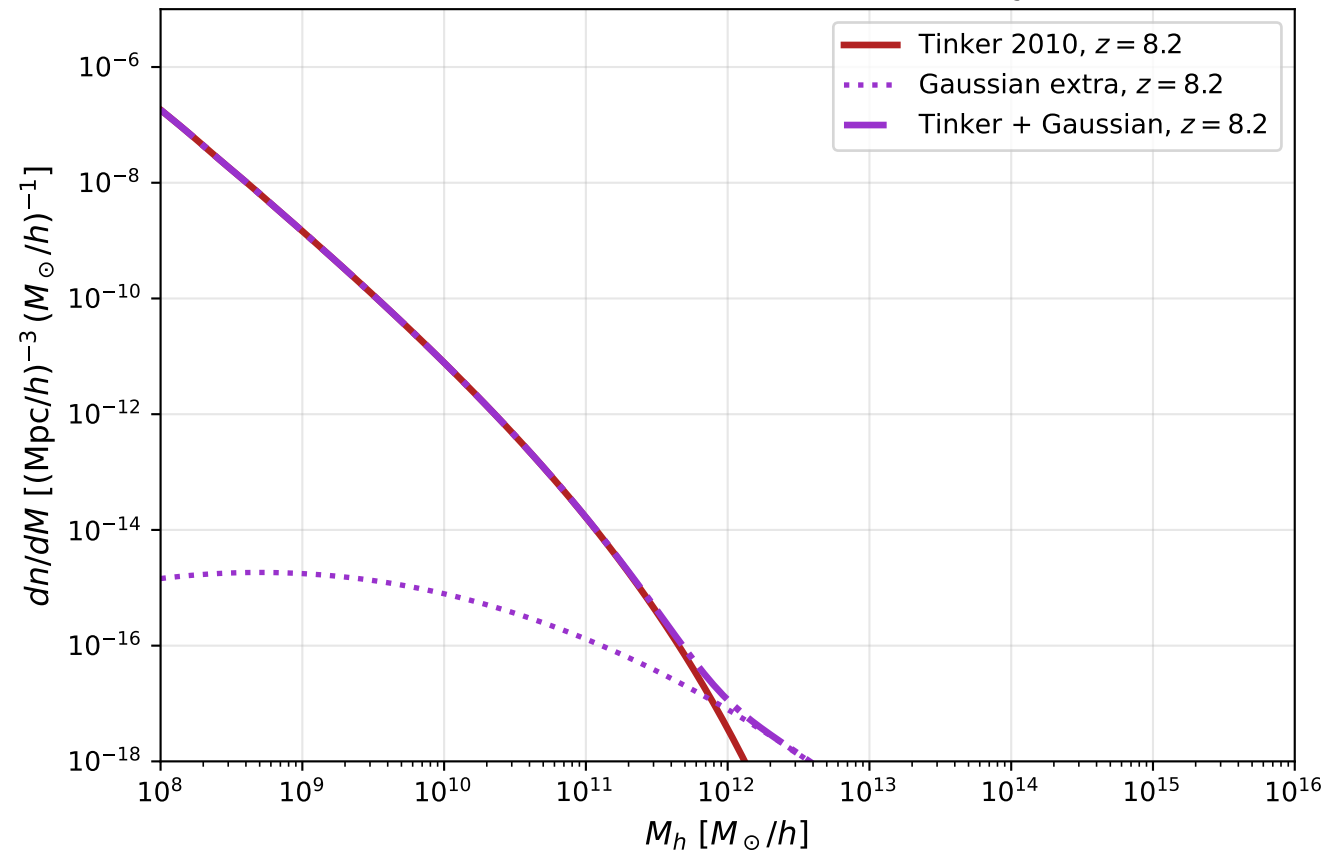
HMF at z = 8.2 : A = 1.3e - 05 , \log M_0 = 11.0 , \sigma_{\log M} = 1.0
