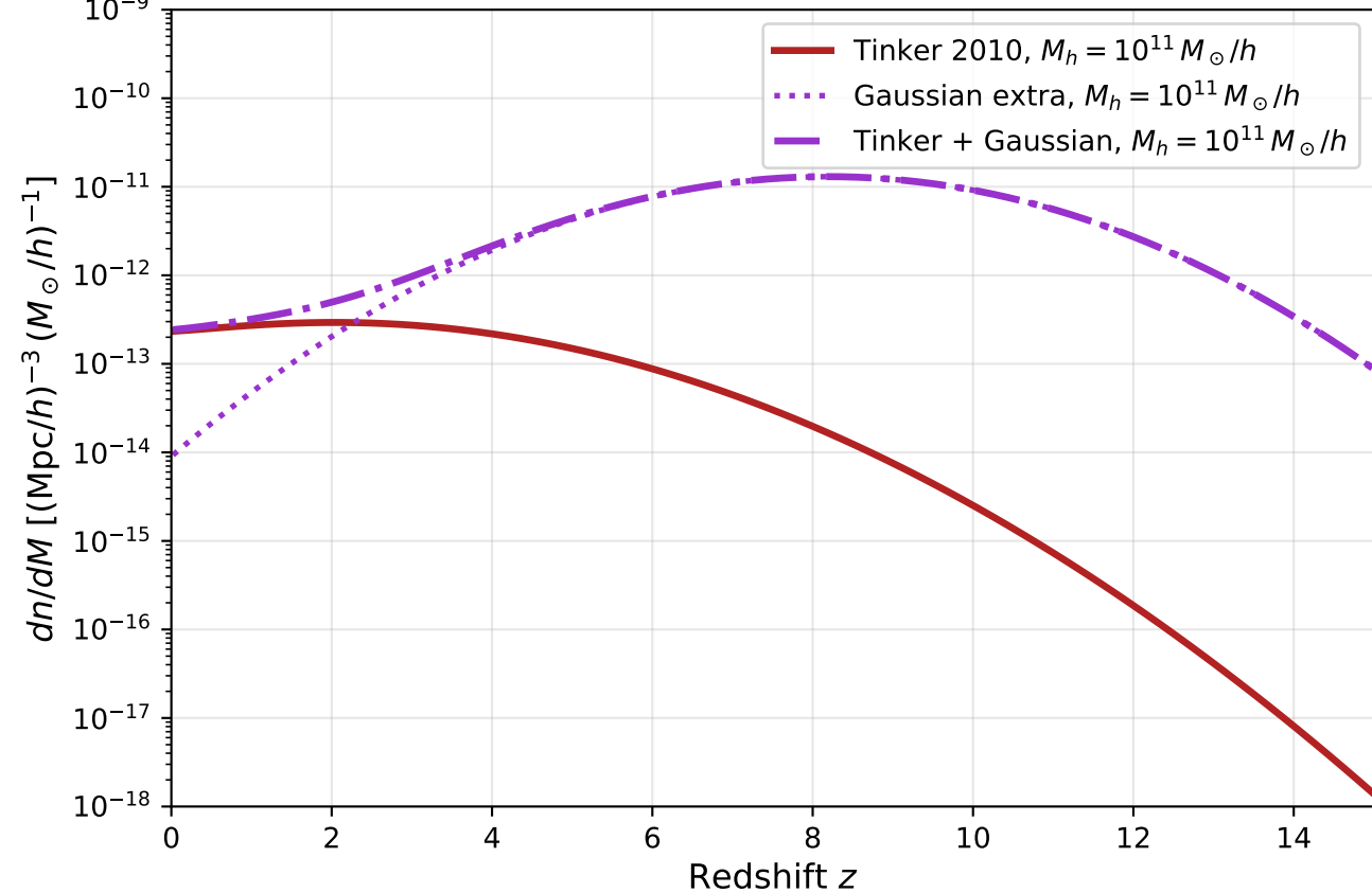
HMF vs z at M_h = 10^{11} M_\odot/h : z_0 = 8.2 , \sigma_z = 2.15
