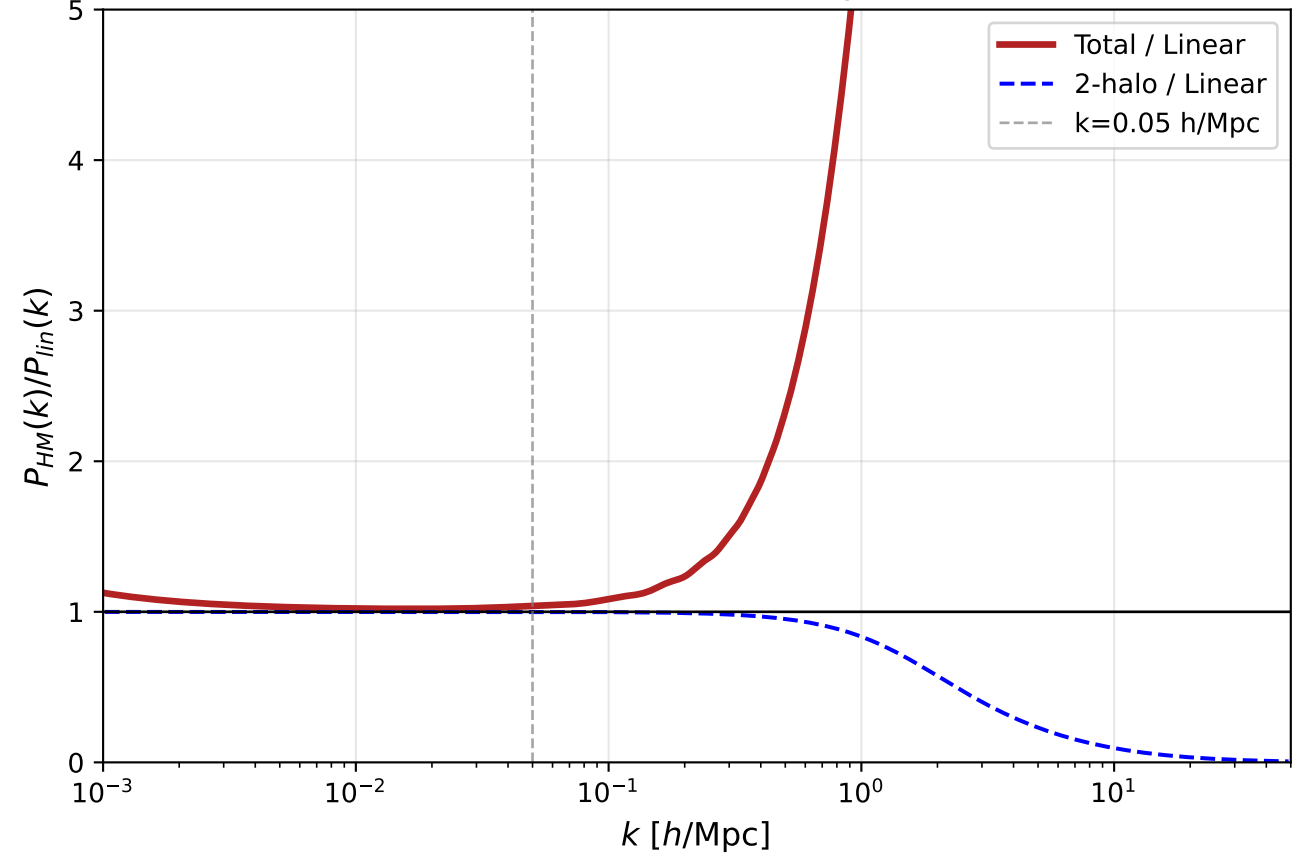
Halo Model / Linear Theory Boost
