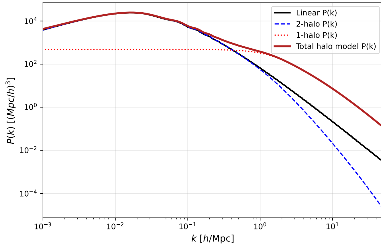
Matter Power Spectrum
