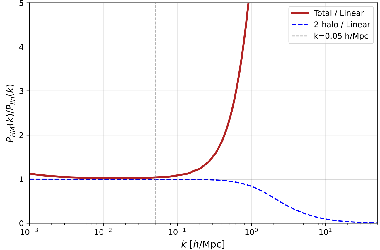
Halo Model / Linear Theory Boost
