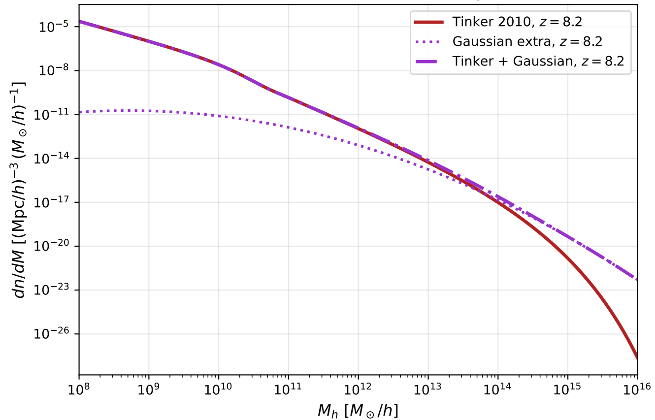
HMF at z = 8.2 : A = 0.3 , \log M_0 = 11.0 , \sigma_{\log M} = 1.0
