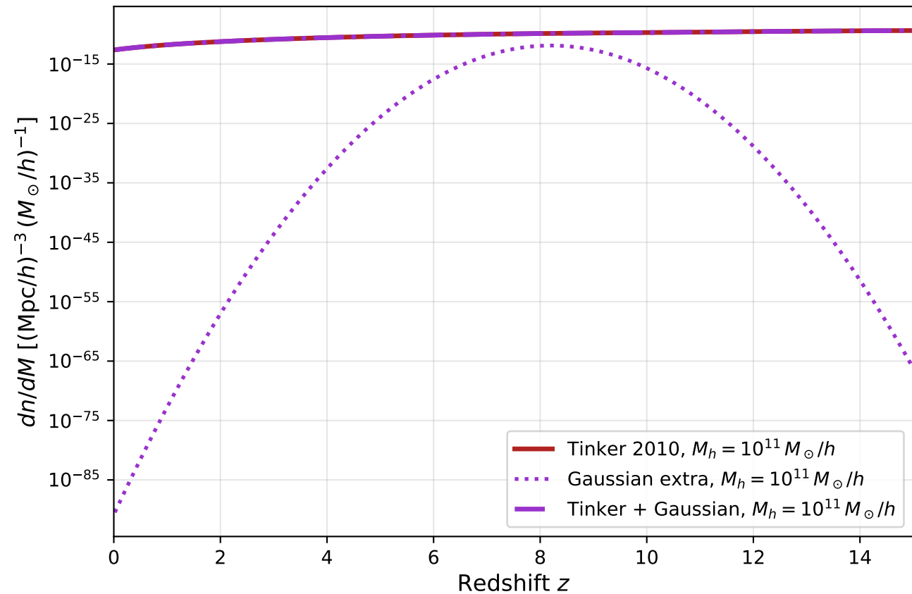
HMF vs z at M_h = 10^{11} M_\odot/h : z_0 = 8.2 , \sigma_z = 0.43
