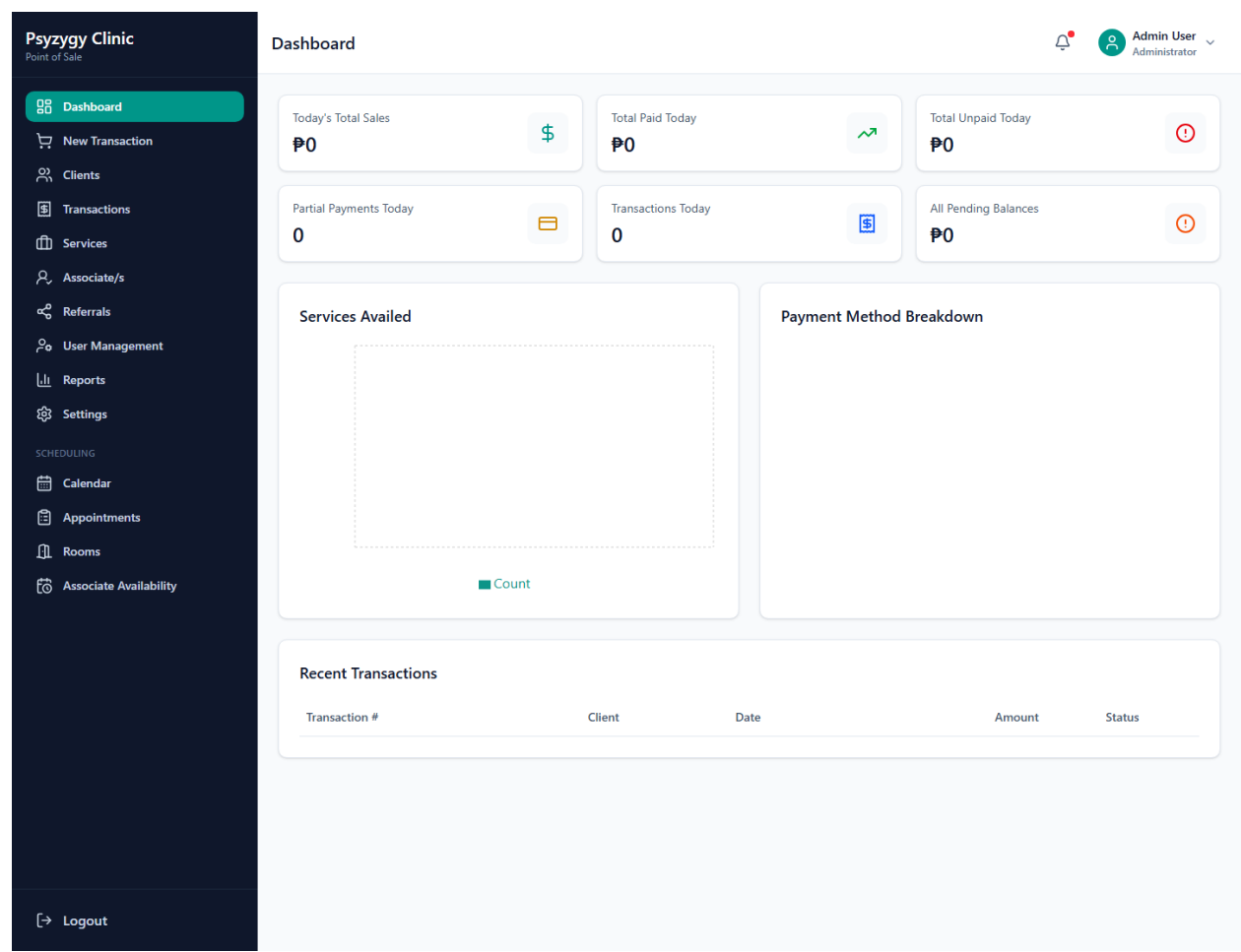
Admin dashboard
