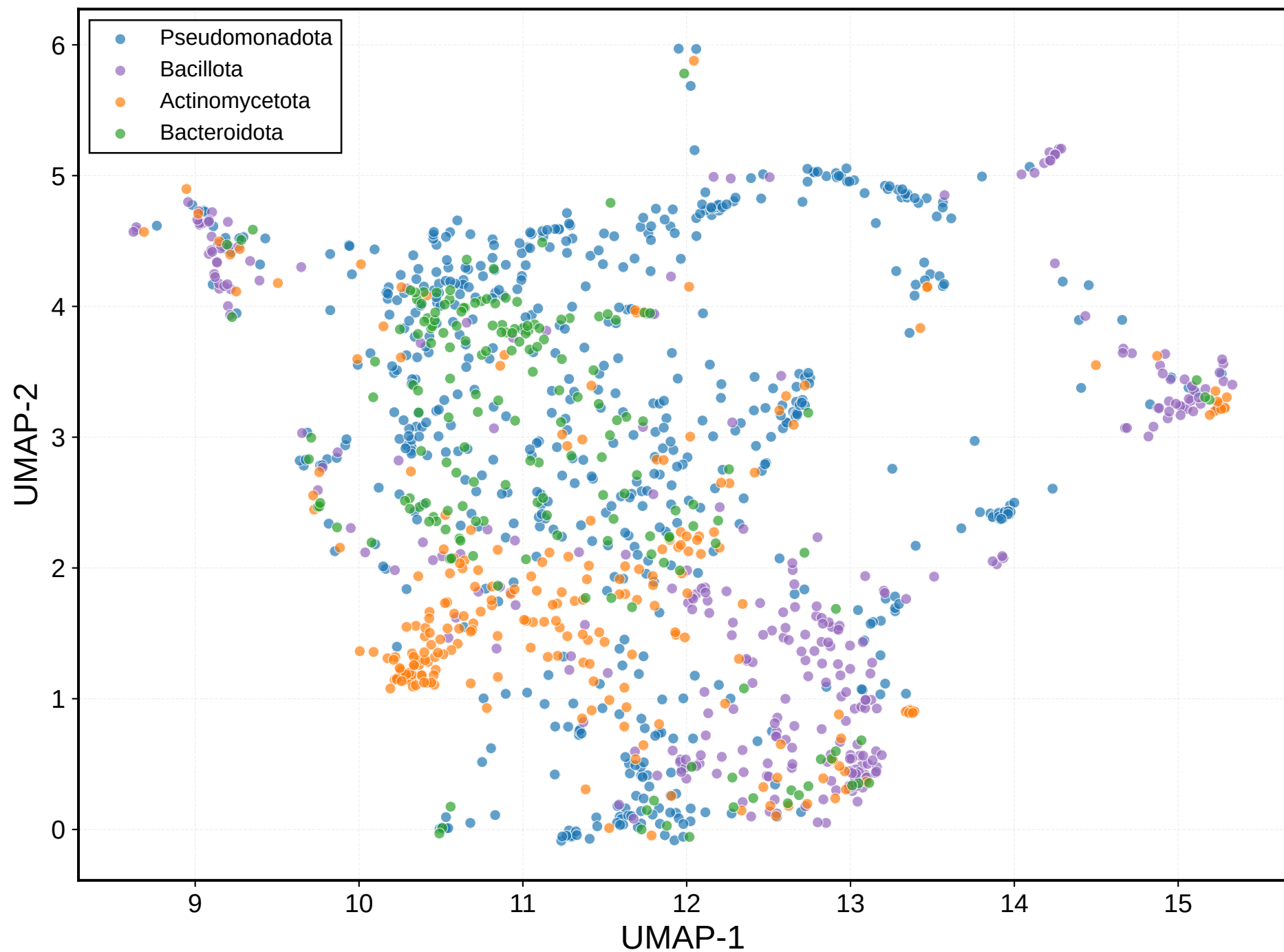
UMAP of Genus Embeddings by Phylum (Main Groups)
