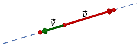
Figura 6: Vectors linealment dependents
