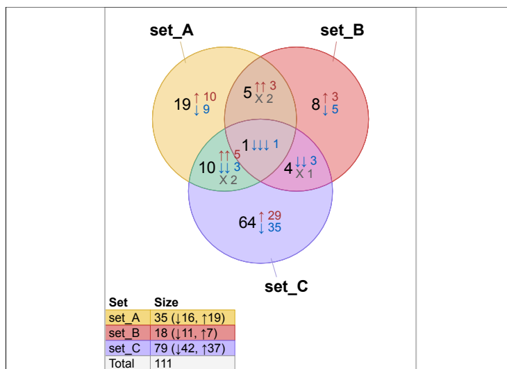
Figure 3.49. Venn diagram with legend in the bottom left corner, adjusted to the bottom edge, and moved more to the left of the figure. The grey box indicates the Venn figure region, the black box indicates the overall figure.
