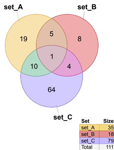
Figure 2.3. Default Venn diagram with three sets, using an incidence matrix as input data.
