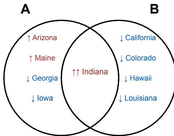
Figure 1.3. Venndir displays the items inside the diagram.
