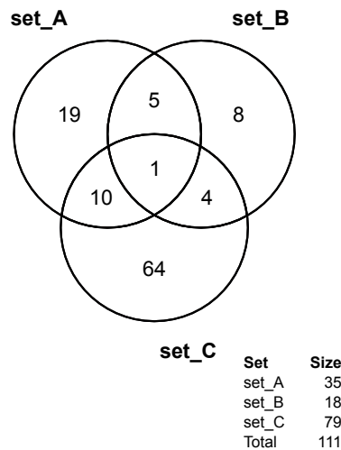
Figure 3.12. Venndir figure with no color.
