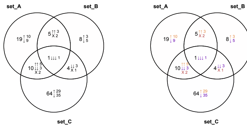
(a) Signed labels in black.
