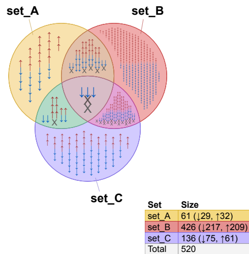
Figure 3.27. Venn diagram showing only the signs of the items filling each overlap region.
