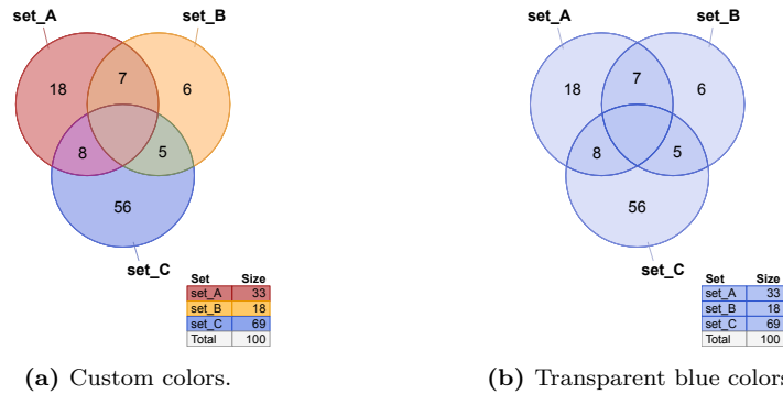
Figure 3.6. Venn diagram showing custom set colors: red, orange, blue.
