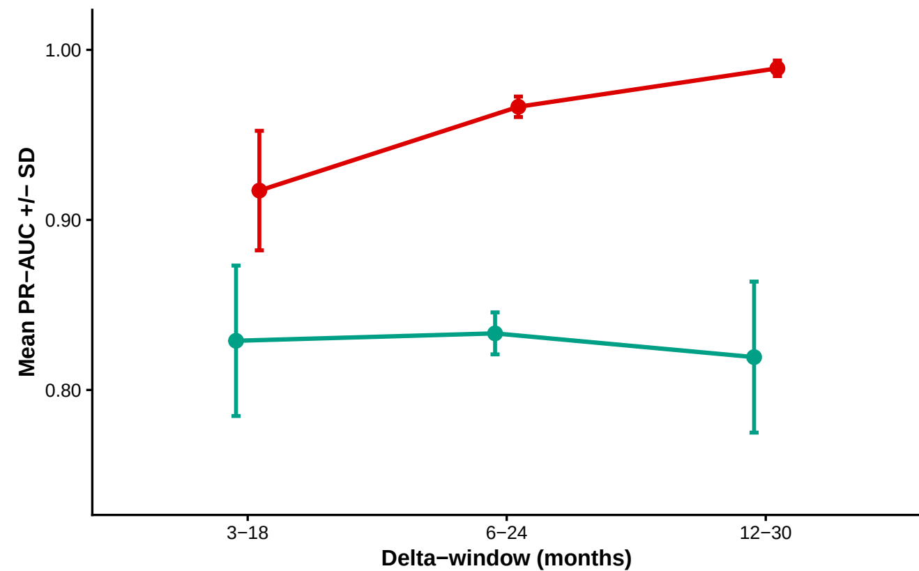
dAUC across windows
