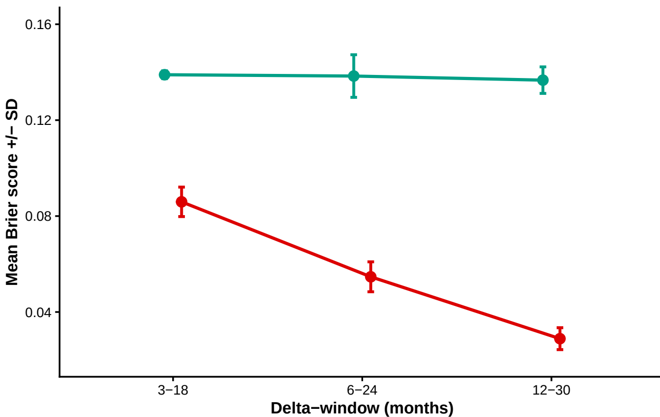
Brier score across windows
