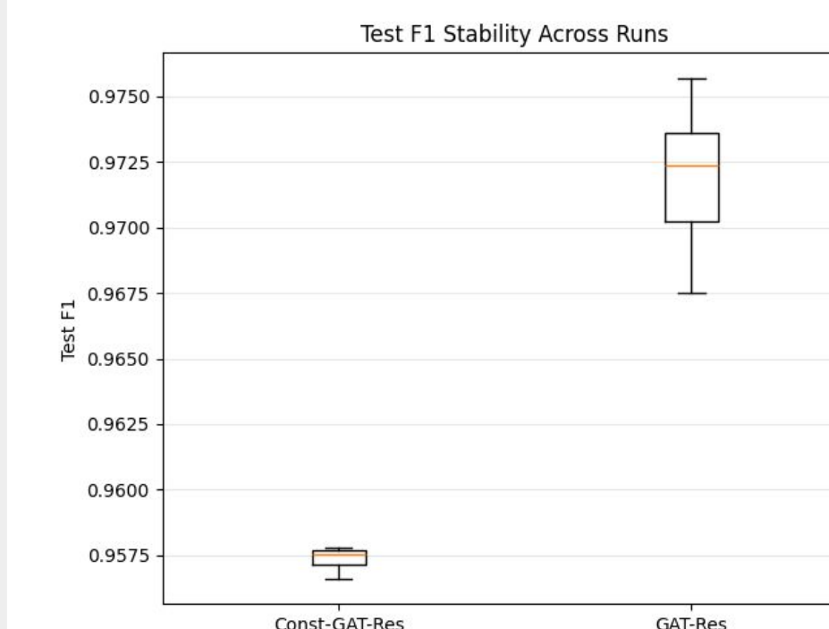
Fig. 5 Test F1 stability across runs showing higher performance and variability for GAT-Res compared to Const-GAT-Res
