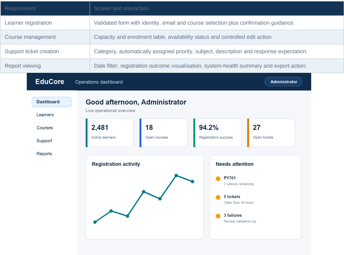
Figure 5. Administrator dashboard and primary navigation.
