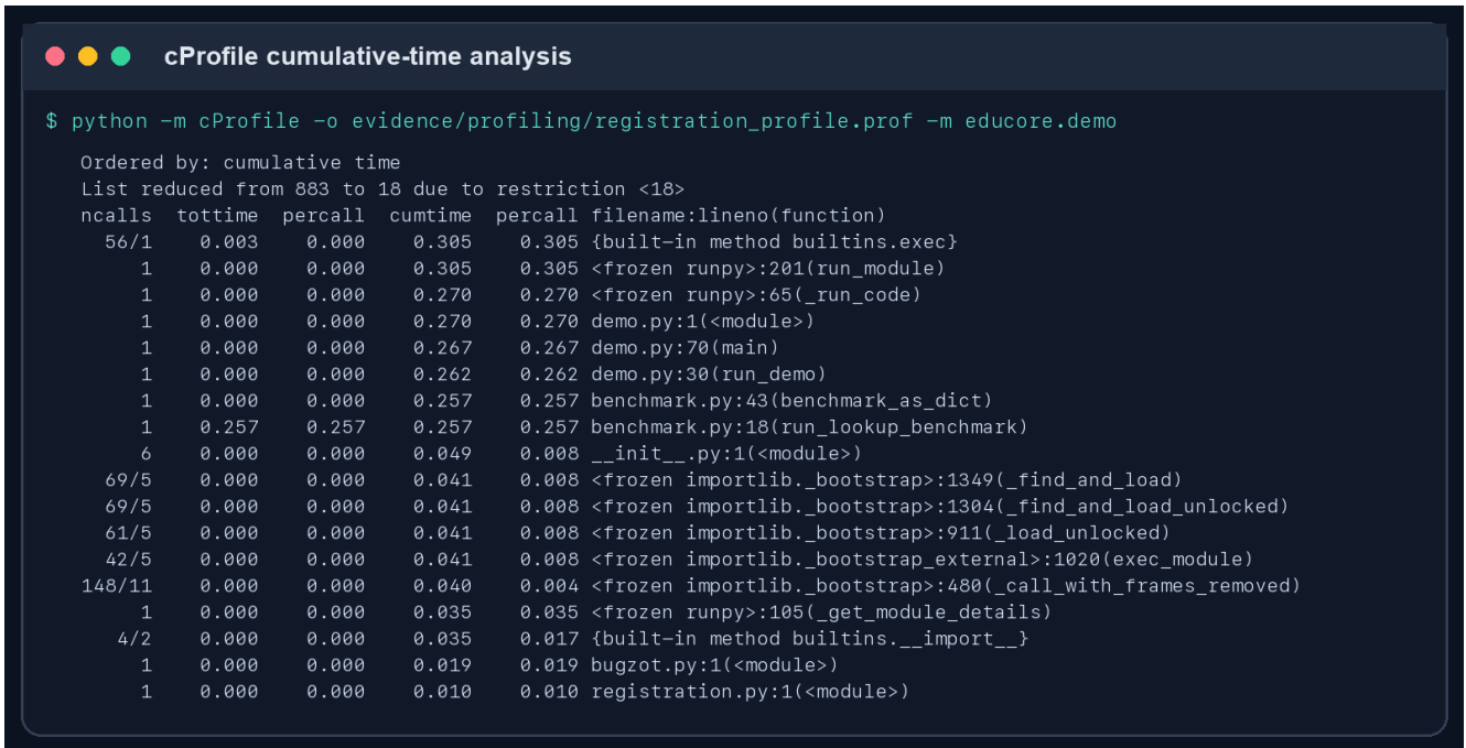
Figure 11. cProfile results sorted by cumulative time.
