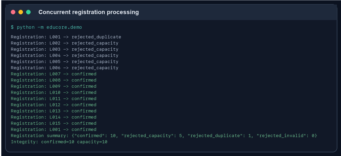
Figure 2. Sixteen concurrent requests produce ten confirmations, five capacity rejections and one duplicate rejection; the final count equals capacity.
