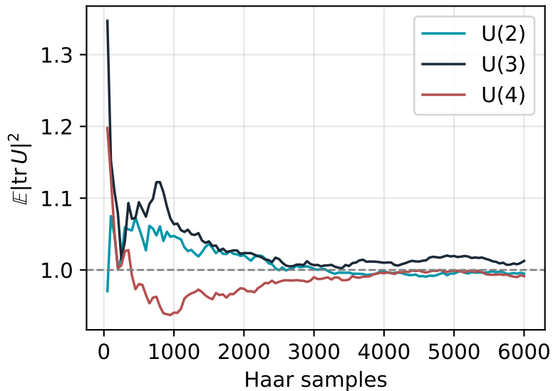
CUE moment convergence
