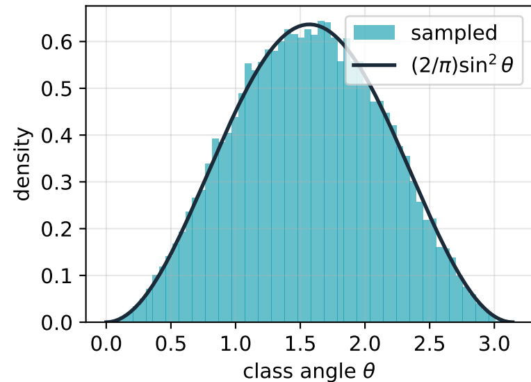
SU(2) Weyl measure
