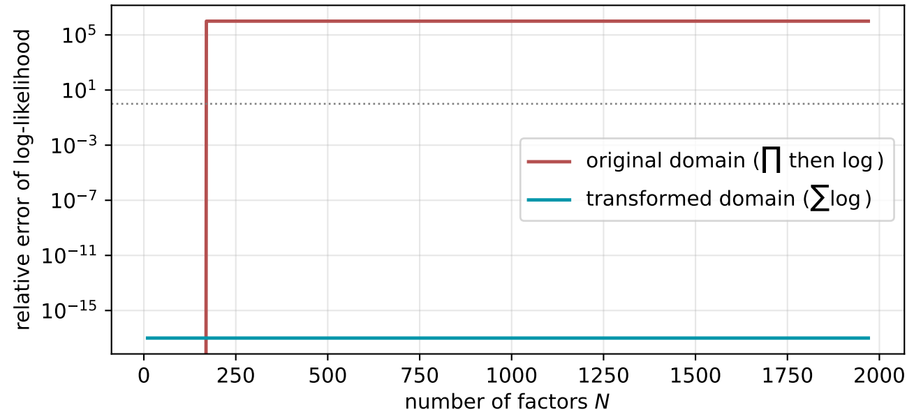
Log-domain stability (underflow of the product)
