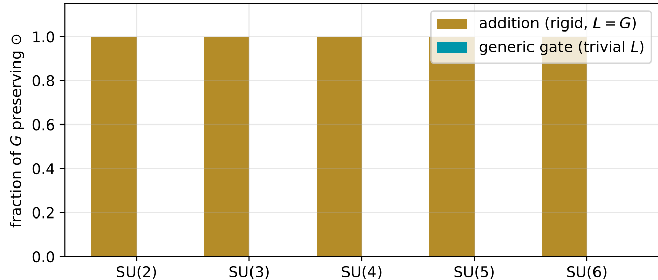
Qudit universality: \text{Op} \cong SU(d) for generic gates
