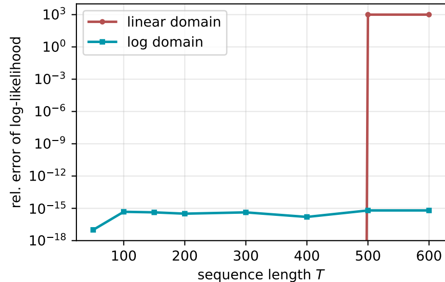
HMM forward: accuracy
