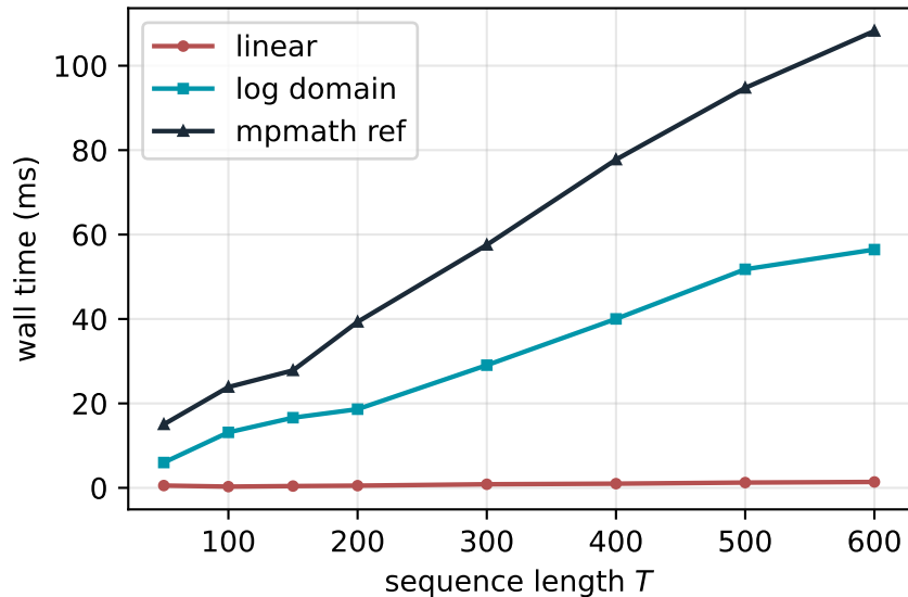
HMM forward: cost
