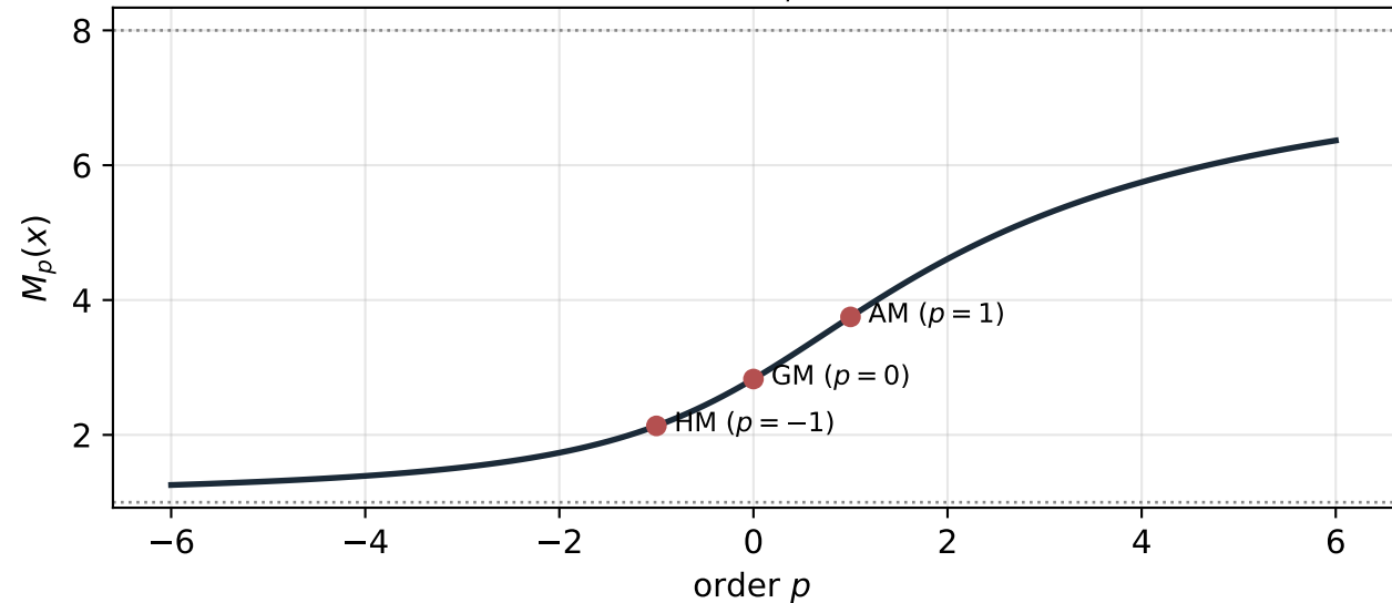
Quasi-arithmetic means: M_p is non-decreasing in p
