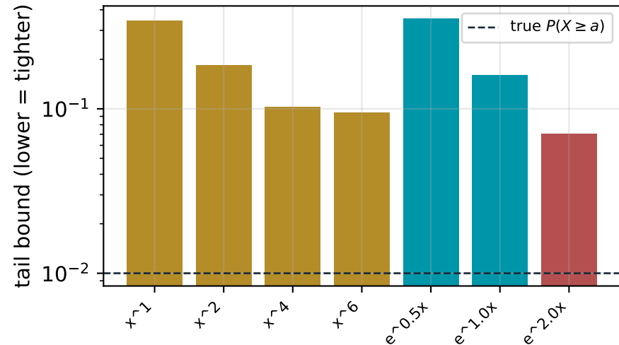
Gaussian (light tail)
