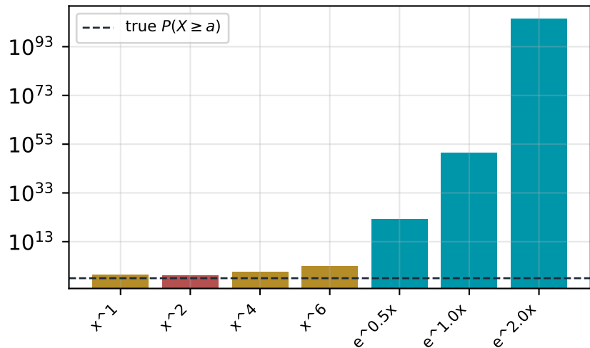
Pareto (heavy tail)
