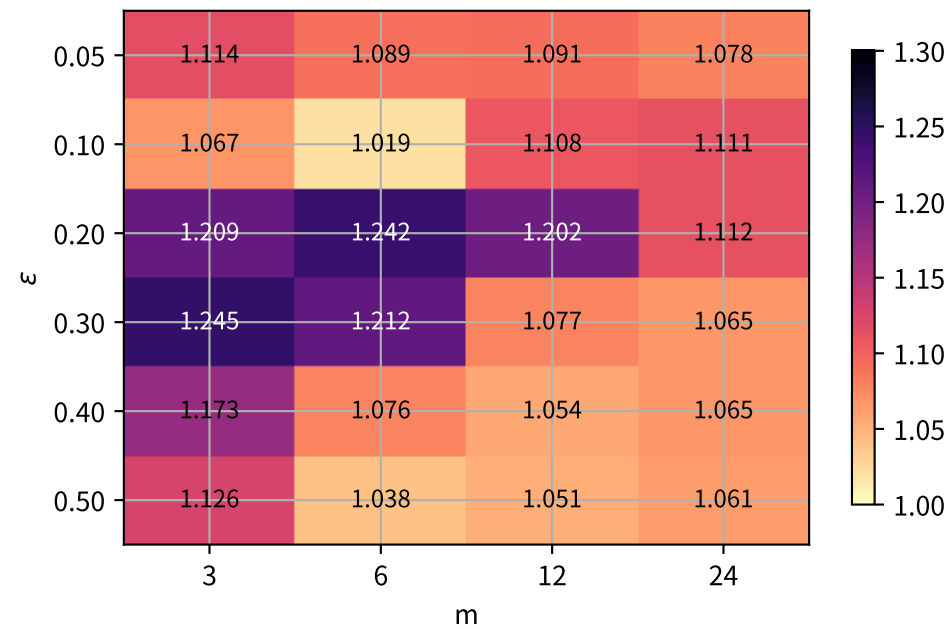
B. \mathbb{R}(\hat{q}^{ho}) / \mathbb{R}(q^{or}) (quantity in Th. S.1.9 )
