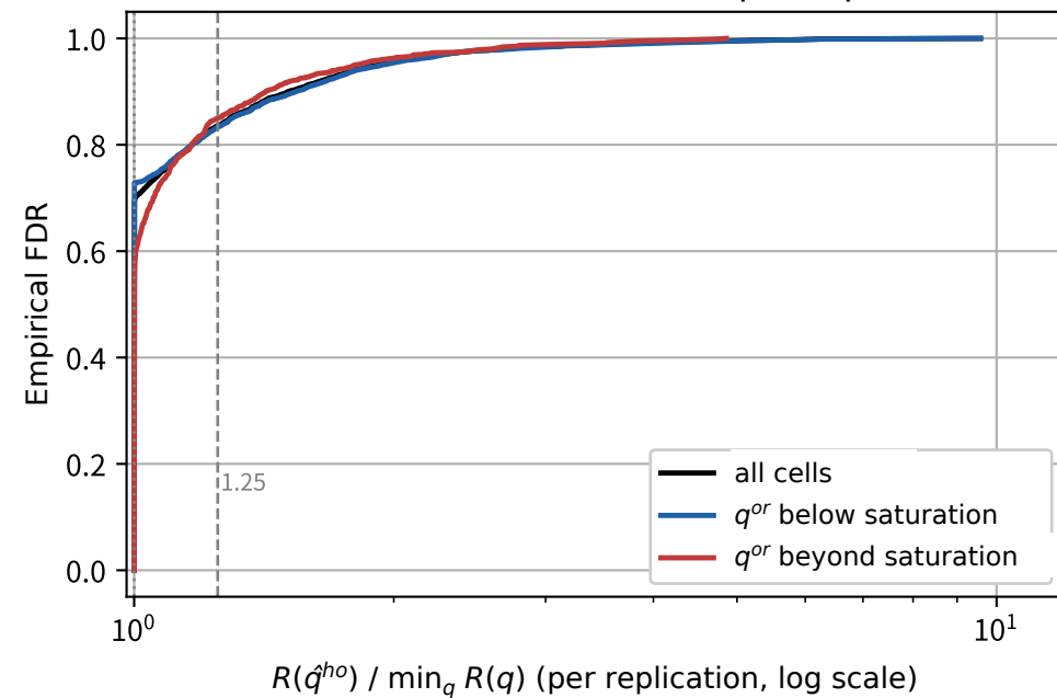
C. Distribution of the risk ratio per replication
