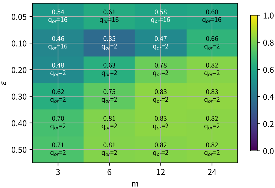
A. Recovery rate \mathbb{P}(\hat{q}^{ho} = q^{or})
