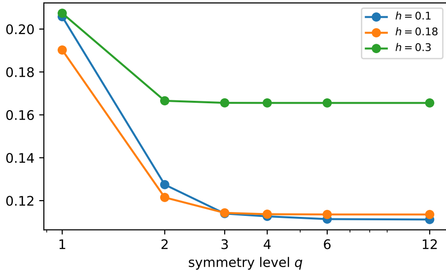
Target: stationary component \Pi_{12}C (gains saturate at the resolution scale)
