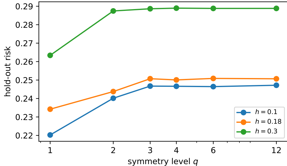
Target: full covariance C (selection refuses symmetry: \hat{q} = 1 )
