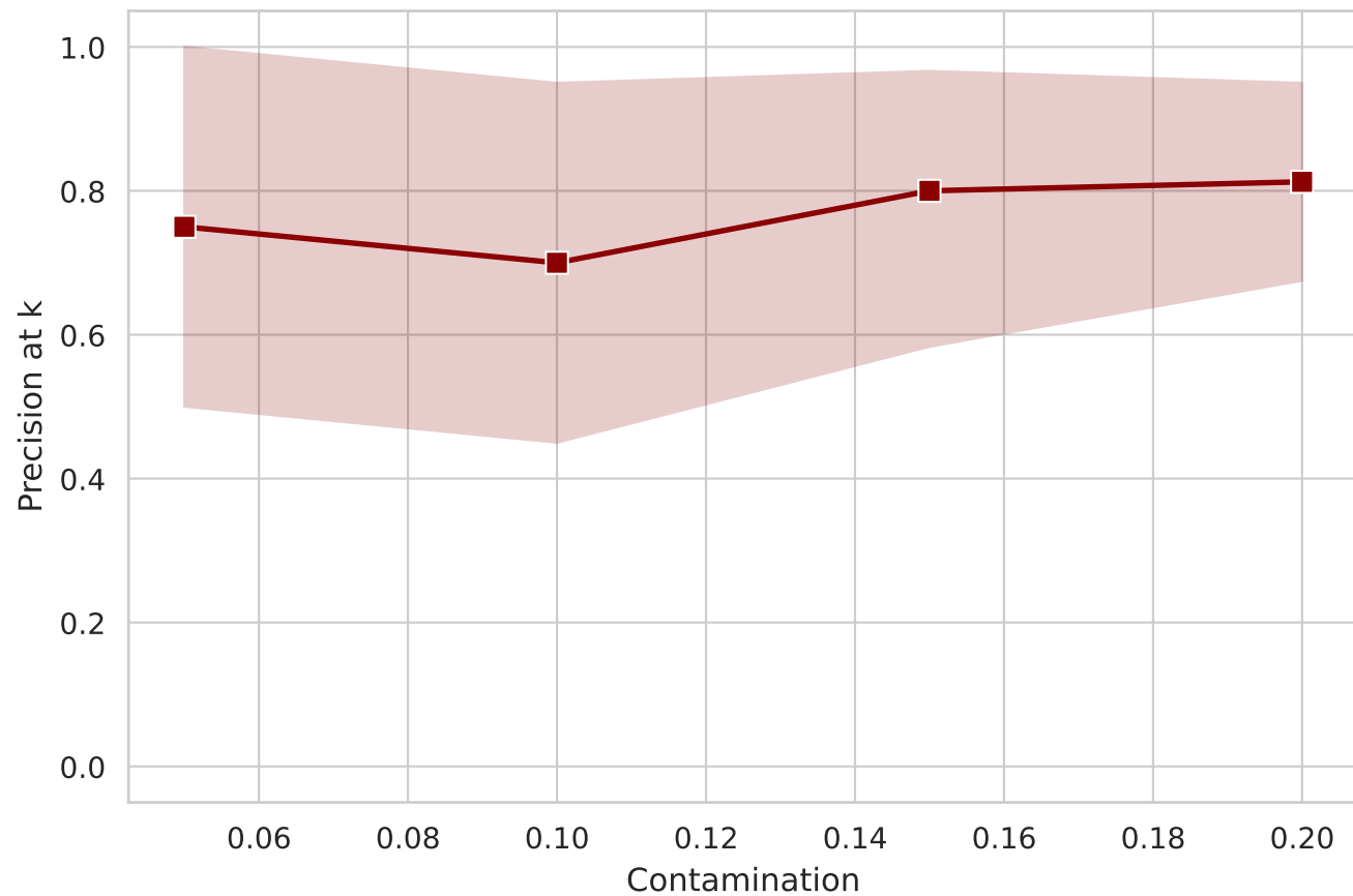
VAE Performance: Precision@k vs contamination
