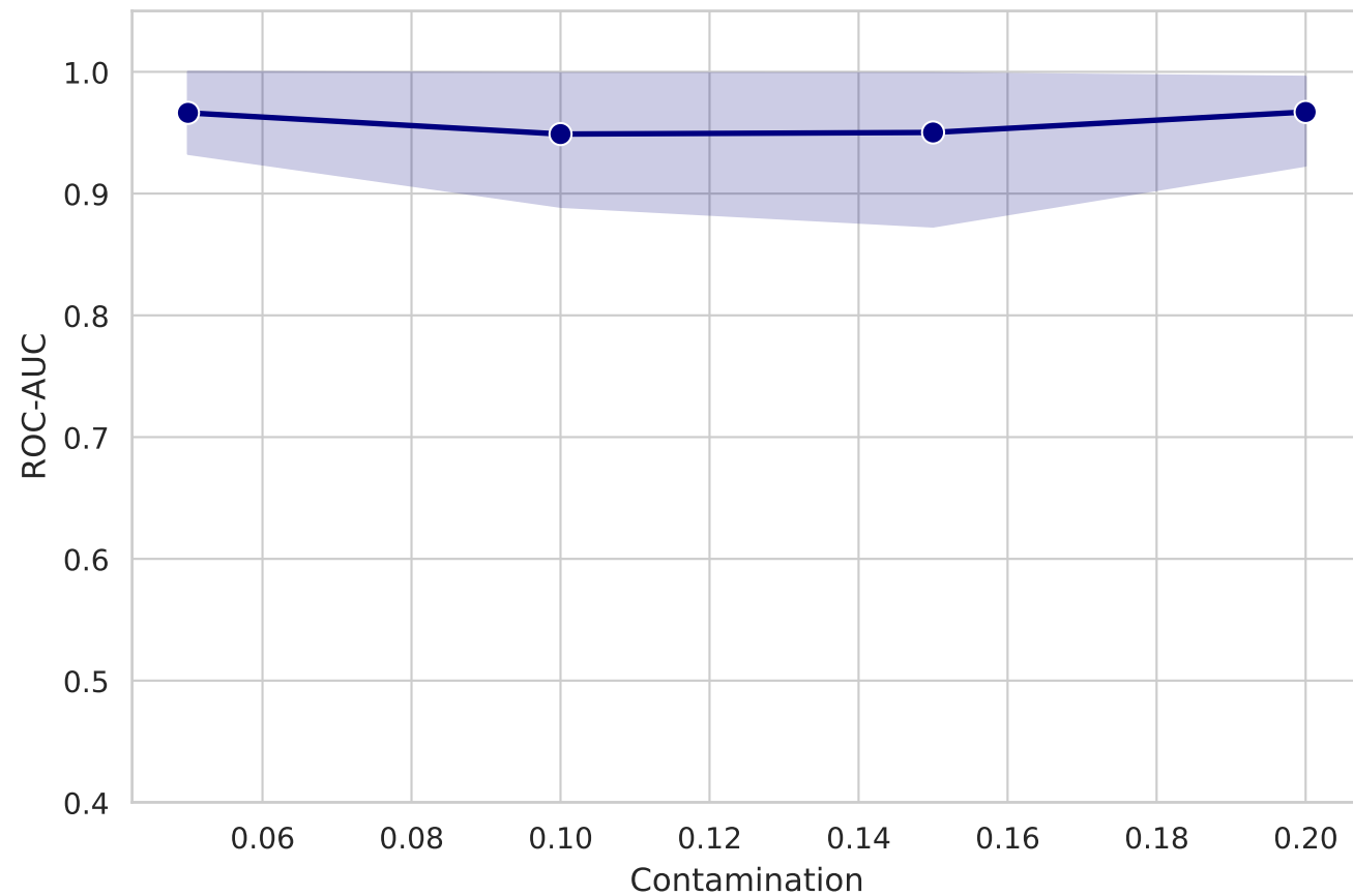
VAE Performance: ROC-AUC vs contamination
