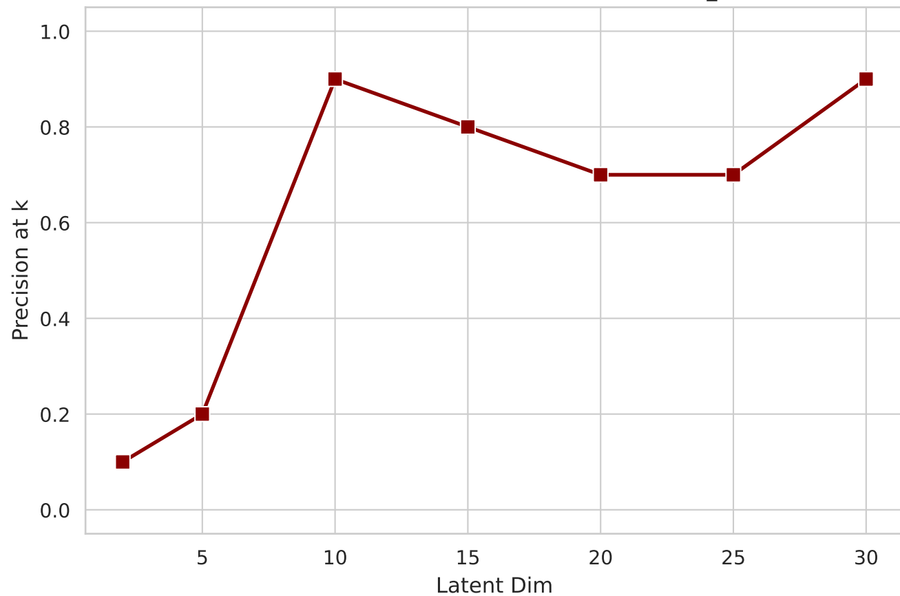
VAE Performance: Precision@k vs latent_dim
