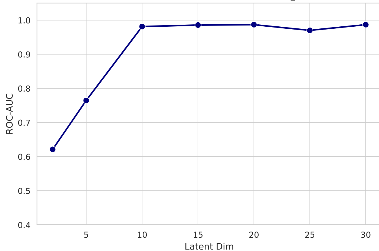
VAE Performance: ROC-AUC vs latent_dim
