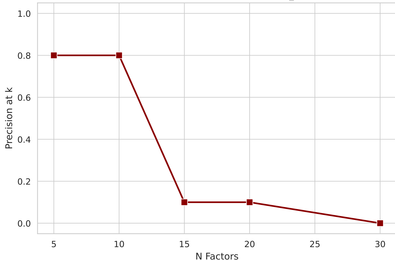
VAE Performance: Precision@k vs n_factors
