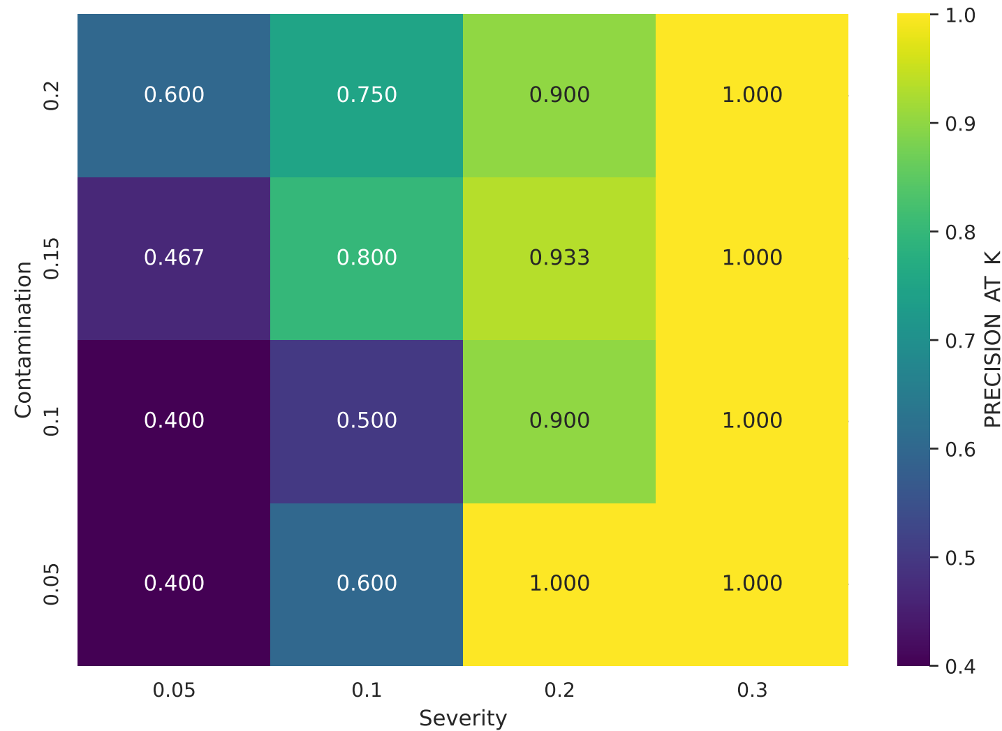
Heatmap: PRECISION_AT_K by severity and contamination
