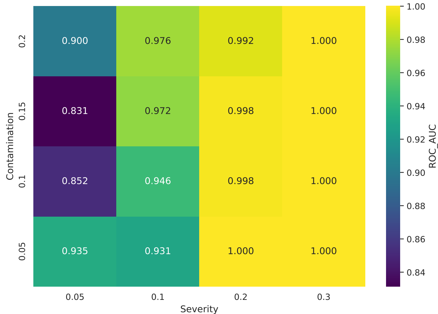
Heatmap: ROC_AUC by severity and contamination
