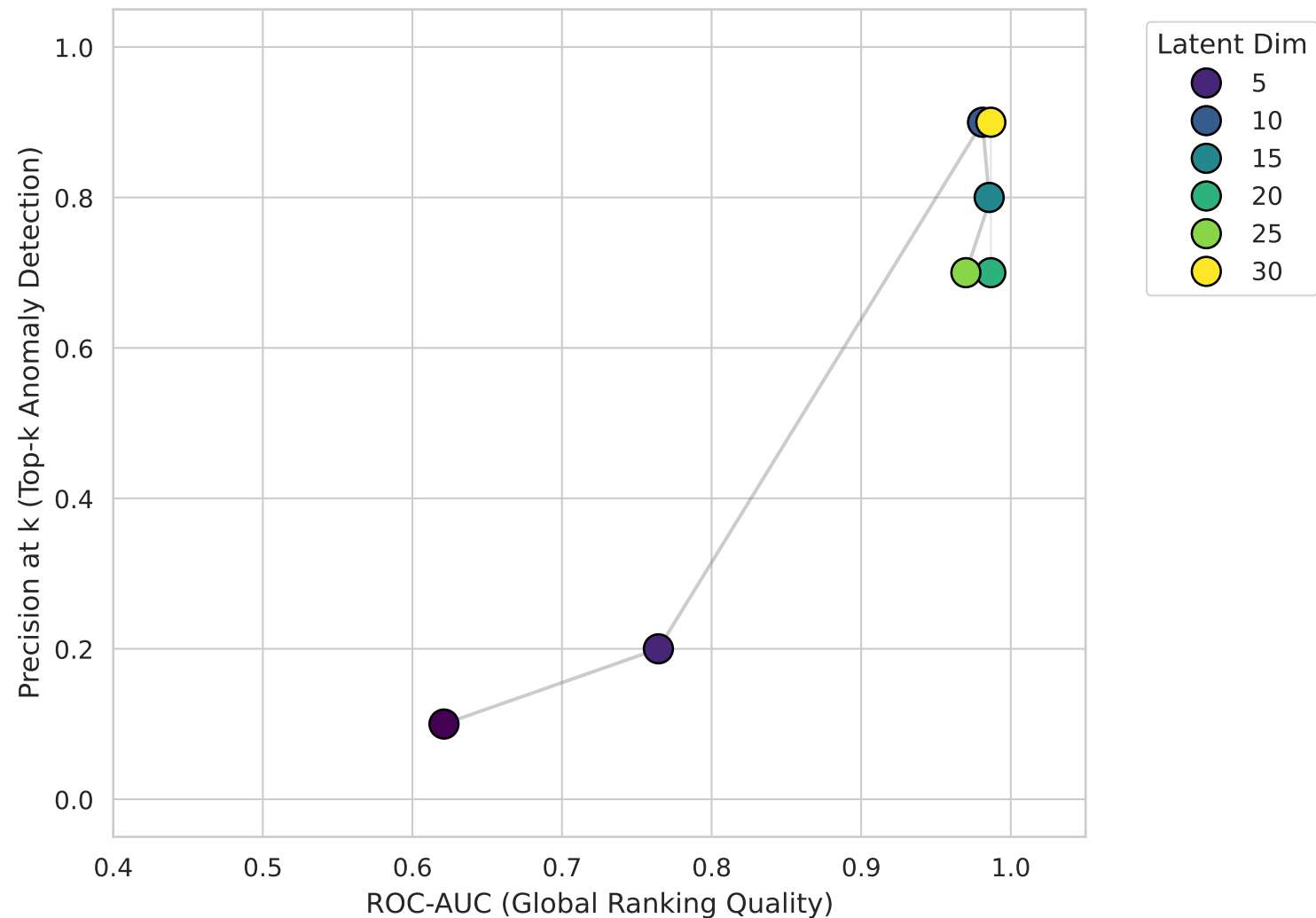
Trade-off Space: Precision@k vs. ROC-AUC
