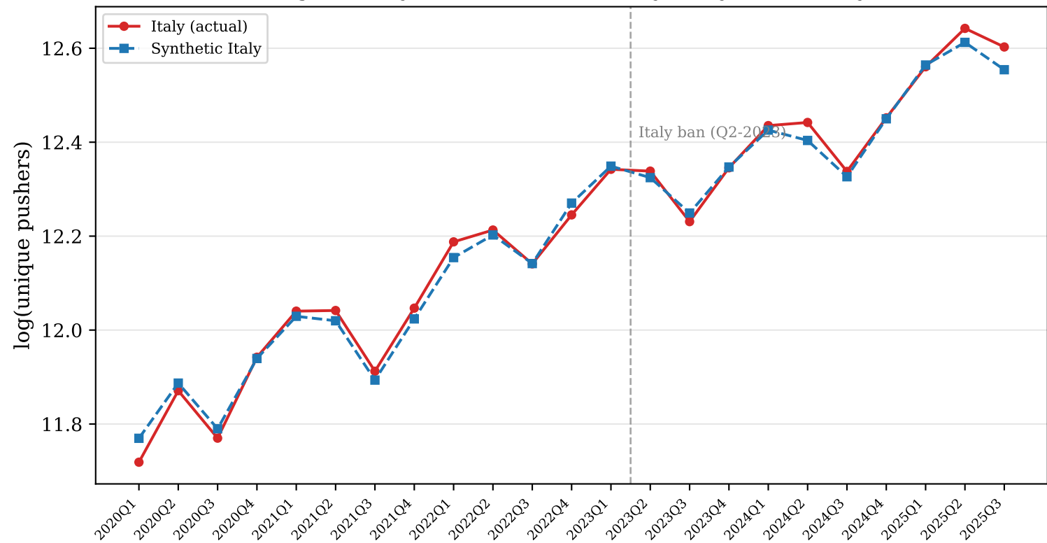
Figure 3: Synthetic Control -- Italy vs Synthetic Italy
