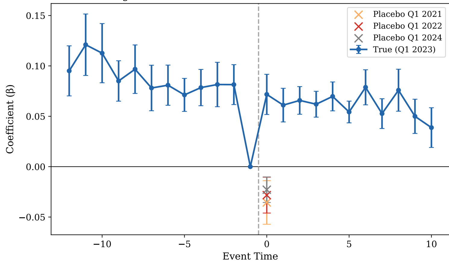
Figure 4: True vs Placebo Treatment Effects on HHI
