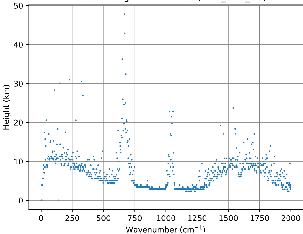
Emission height at \tau = 1 for (H2O_CO2_O3)
