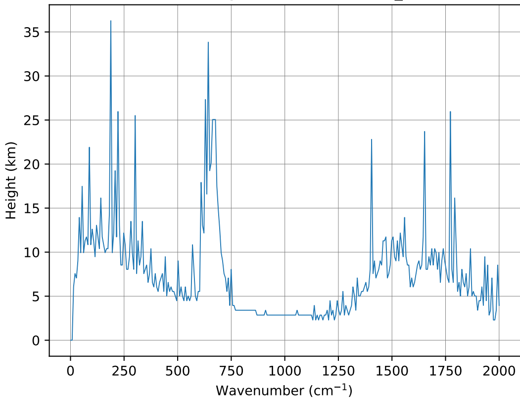
Emission height at \tau = 1 for (H 2 O_CO 2 )
