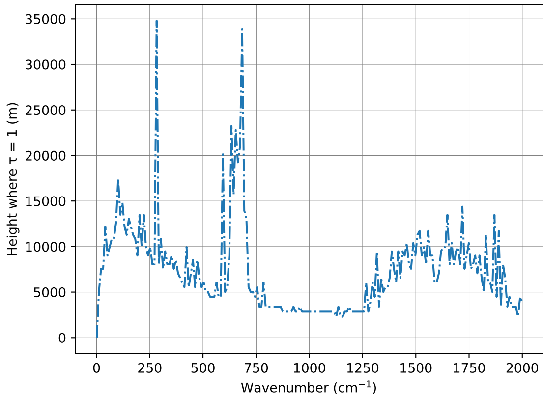
Emission height ( \tau = 1 ) vs. wavenumber
