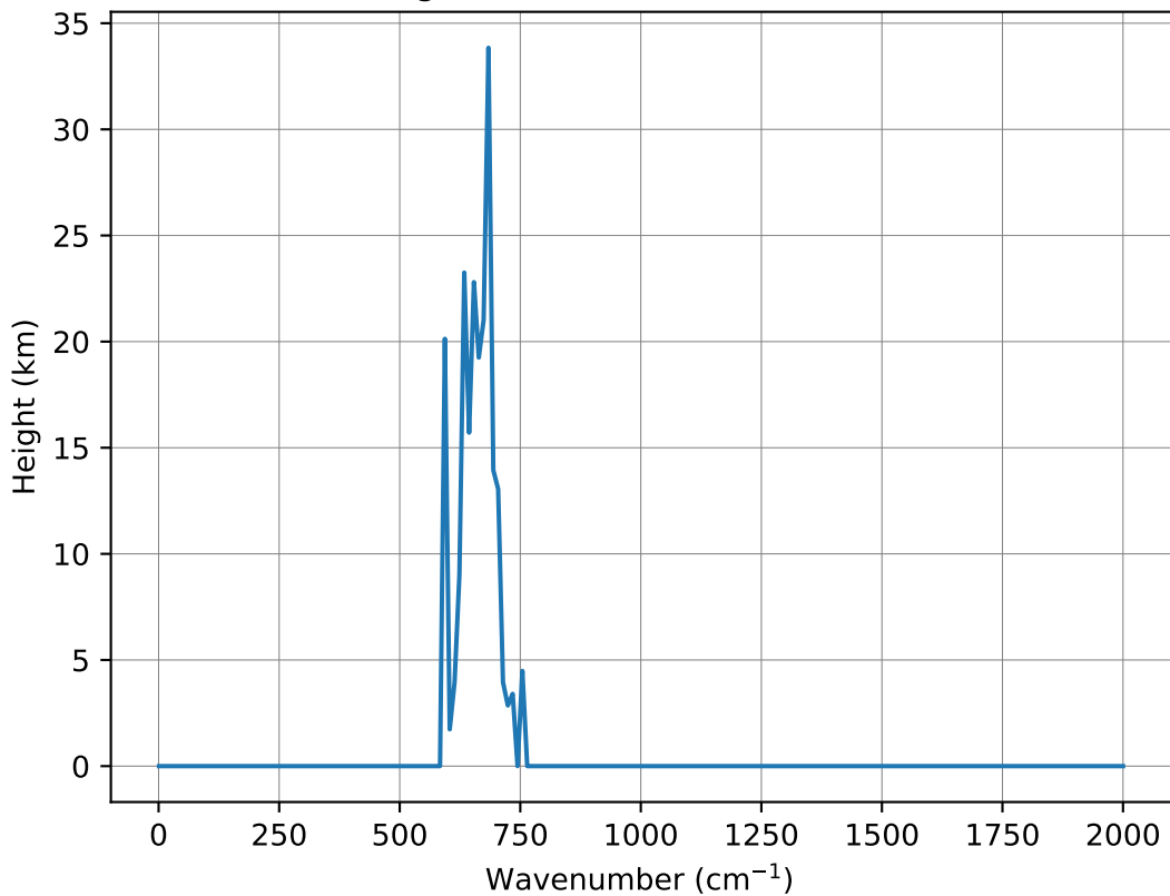
Emission height ( \tau = 1 ) vs. wavenumber for (CO 2 )
