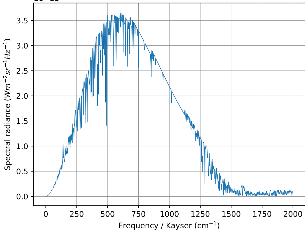
Planck emission at \tau = 1 level for (H 2 O)
