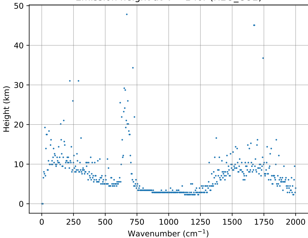
Emission height at \tau = 1 for (H 2 O_CO 2 )
