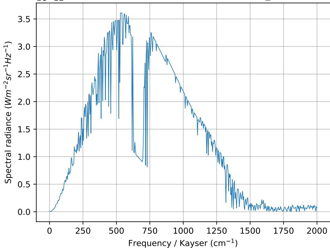
1e-12 Planck emission at \tau = 1 level for (H2O_CO2)
