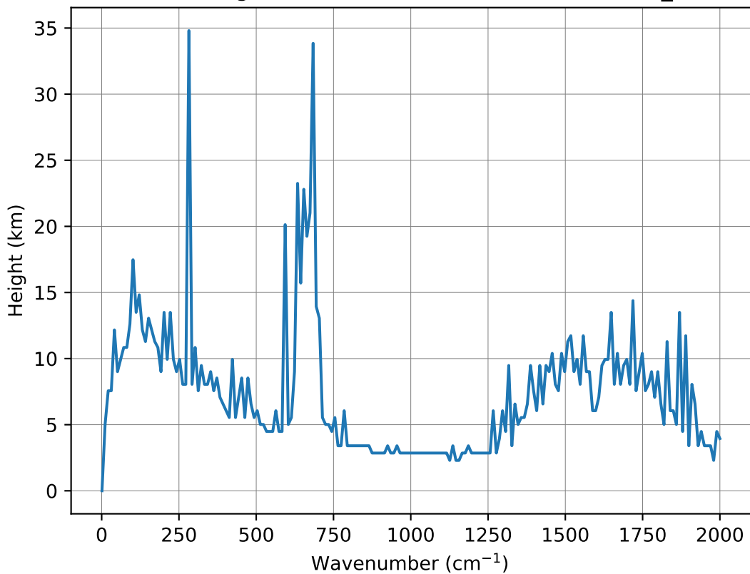
Emission height ( \tau = 1 ) vs. wavenumber for (H 2 O_CO 2 )
