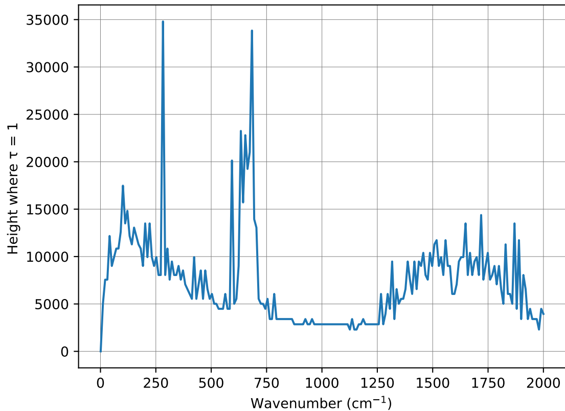
Emission height ( \tau = 1 ) vs. wavenumber for H 2 O and CO 2
