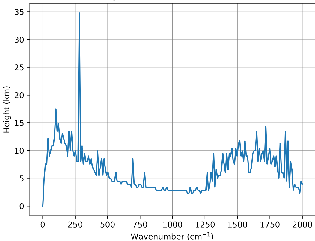
Emission height ( \tau = 1 ) vs. wavenumber for (H 2 O)
