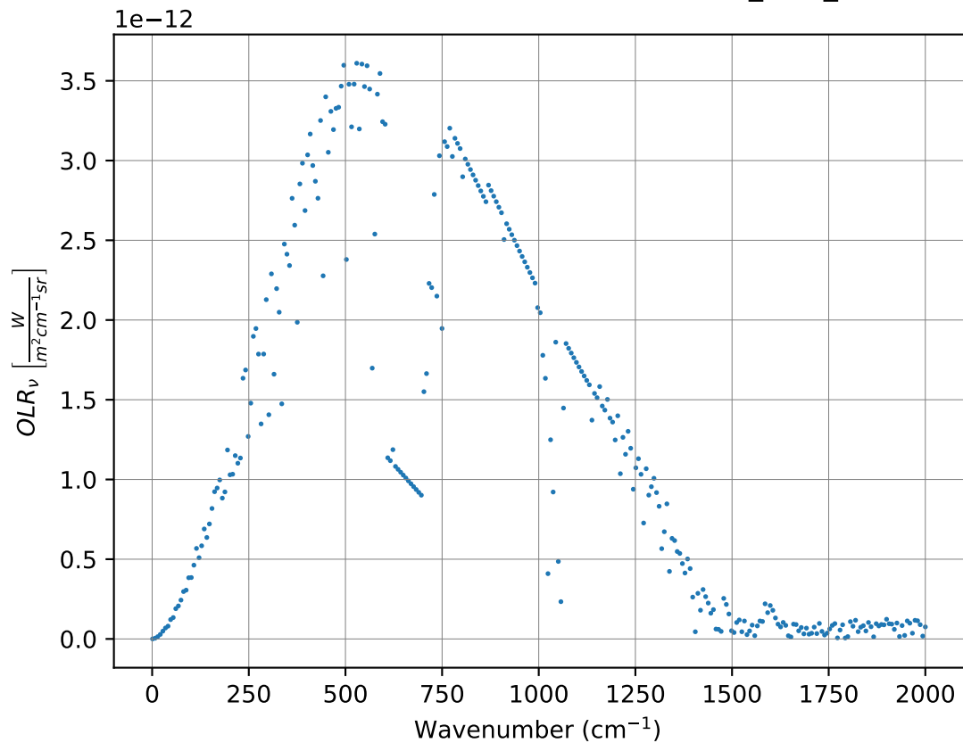
Planck emission at \tau = 1 level for (H2O_CO2_O3)
