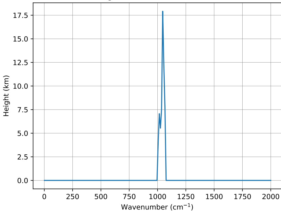
Emission height ( \tau = 1 ) vs. wavenumber for (O3)
