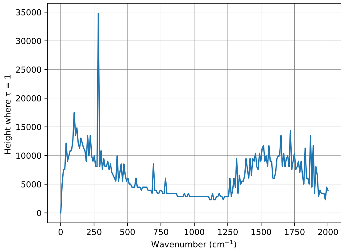
Emission height ( \tau = 1 ) vs. wavenumber for CO 2
