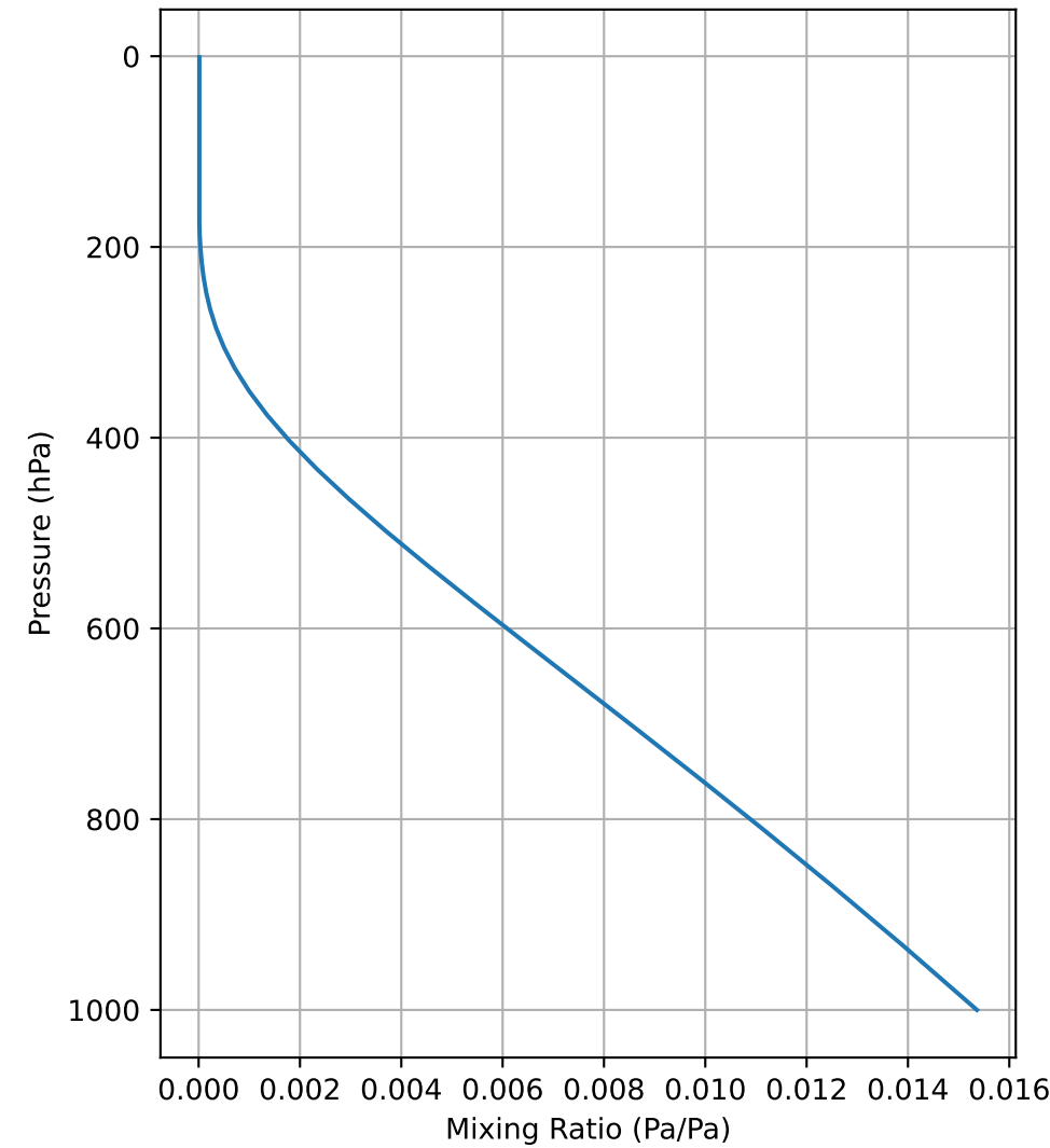
Water Vapor VMR
