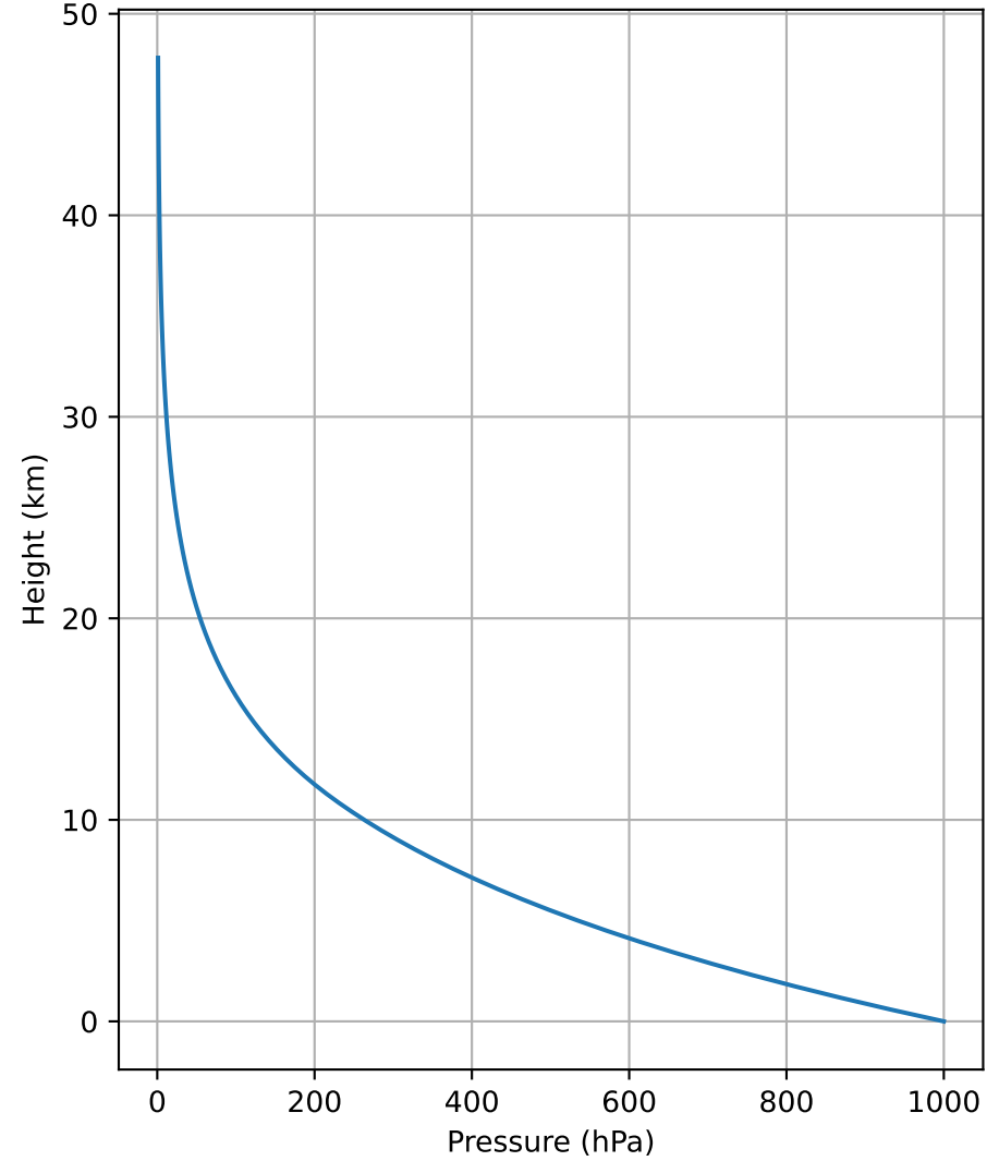
Pressure profile
