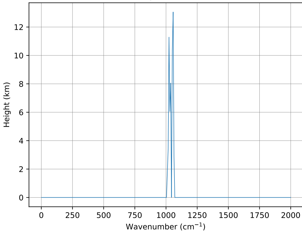
Emission height at \tau = 1 for (O3)
