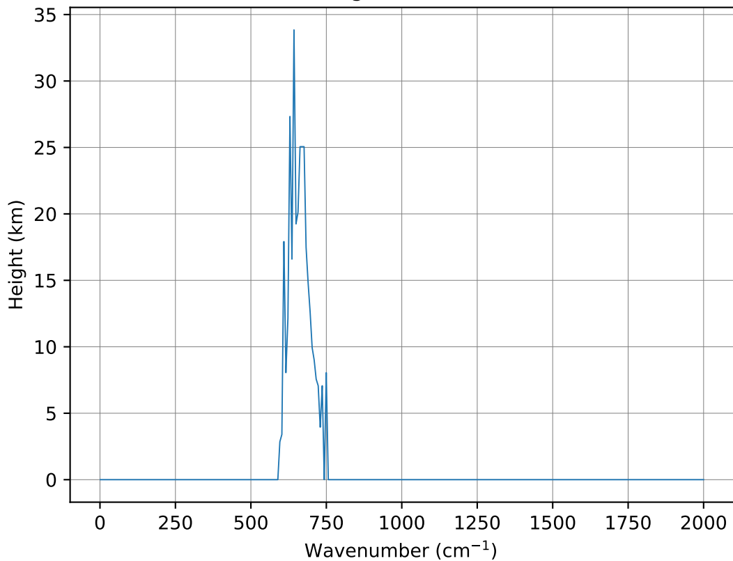
Emission height at \tau = 1 for (CO 2 )
