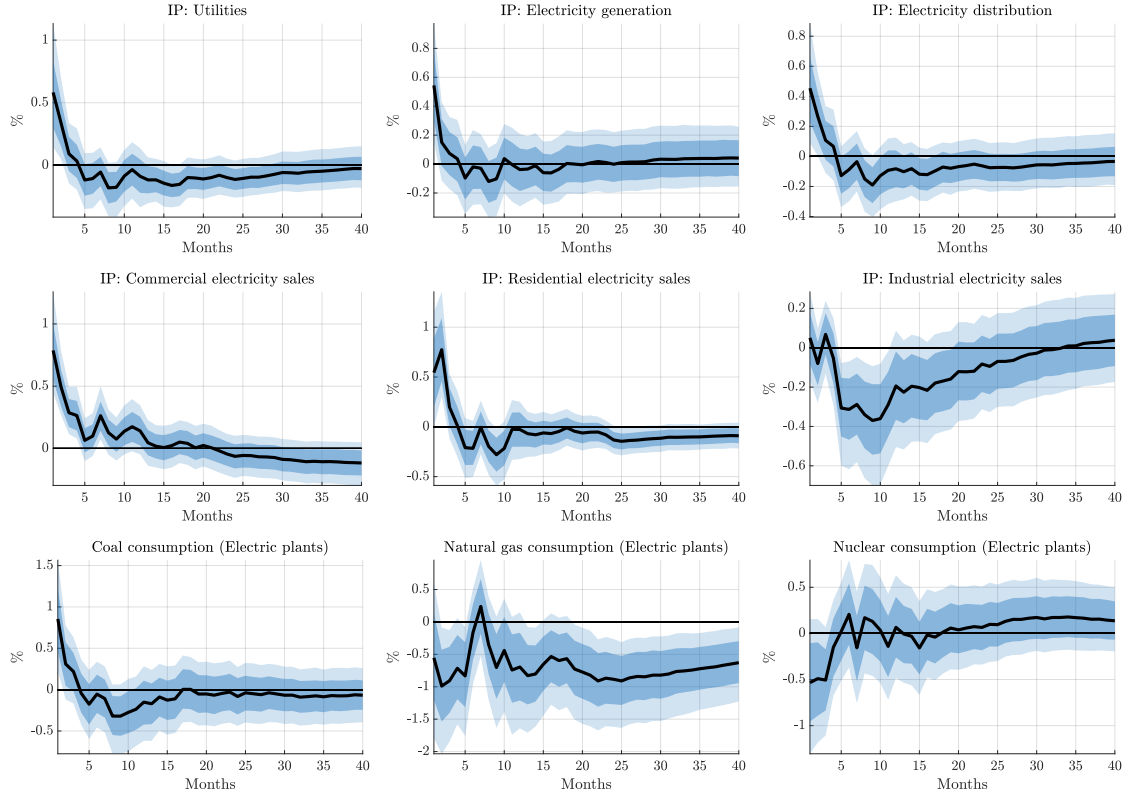
Figure 12: Impulse responses to a monetary policy tightening:: Electricity generation and sales
