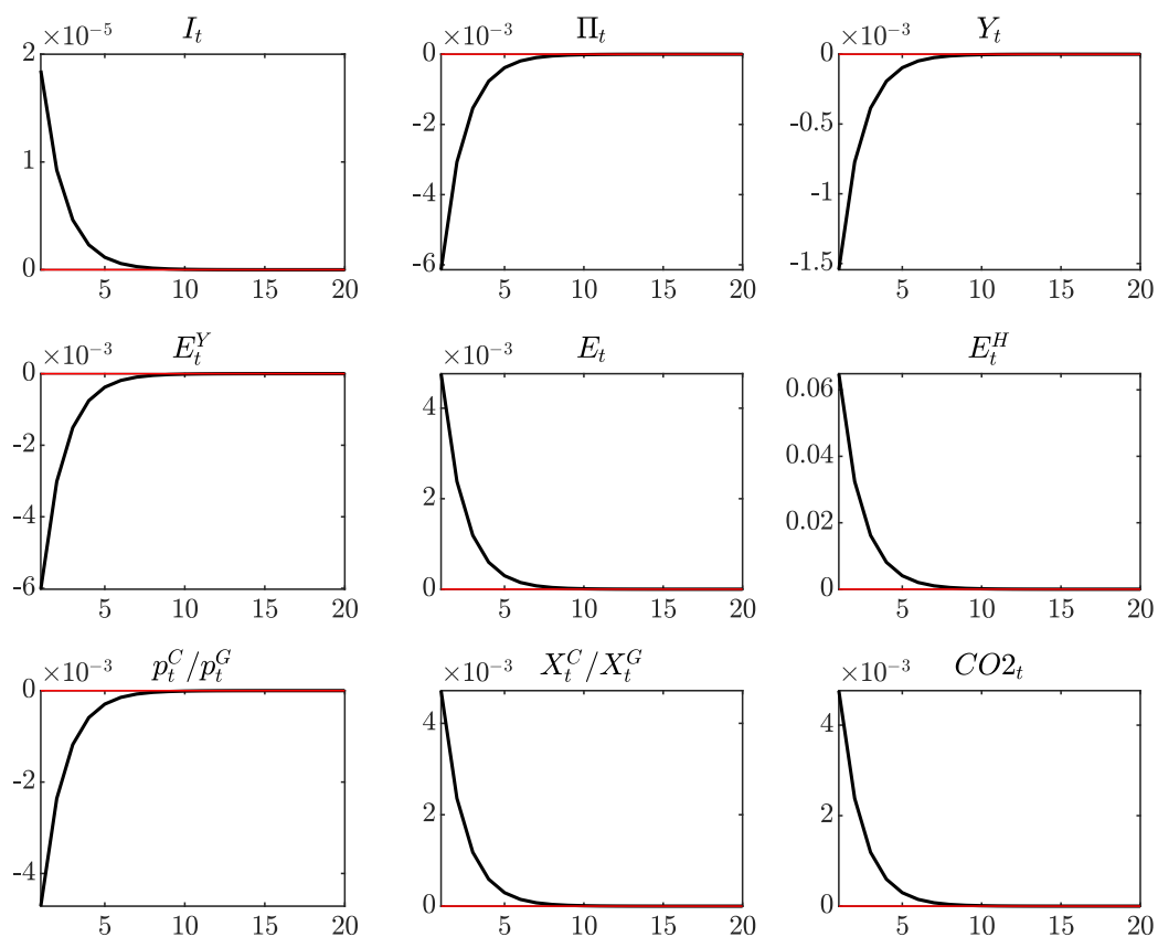
Figure A.3: Dynamic responses to a technology shock: Interest rate rule
