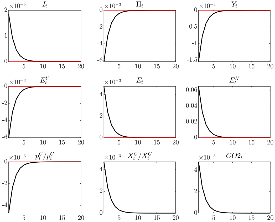
Figure 15: Dynamic responses to a monetary policy shock: Interest rate rule
