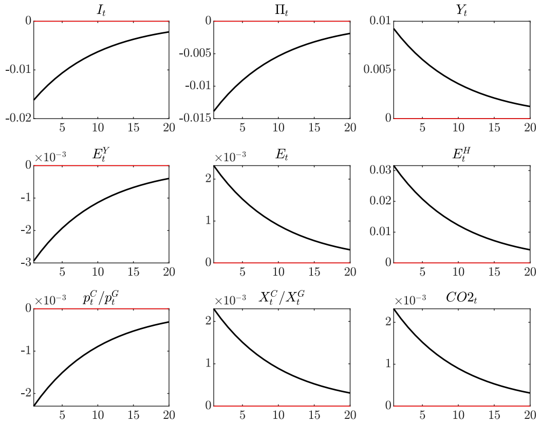
Figure A.8: Dynamic responses to a technology shock: Interest rate rule
